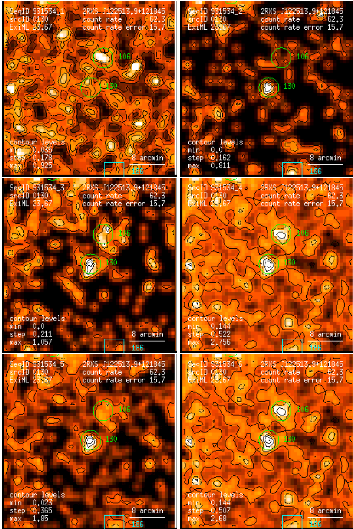
Figure 130: RASS 931534: detection 0130: band rate images, Gaussian filter: (1) PSPC channels 11 – 41, (2) 52 – 90, (3) 91 – 201, (4) 11 – 235, (5) 52 – 201, (6) 11 – 201. Broad band rates in counts/ks. Band rate contour levels in counts/ks/arcmin 2 .
