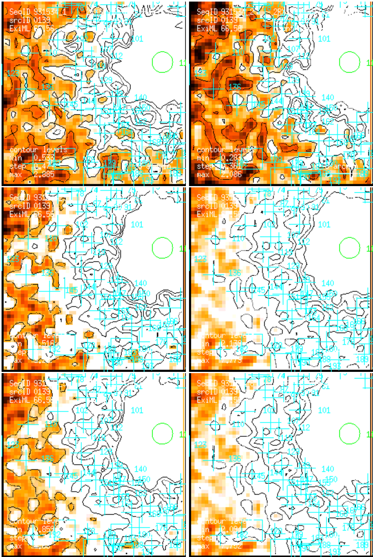
Figure 139: RASS 931534: detection 0139: band rate images, Gaussian filter: (1) PSPC channels 11 – 41, (2) 52 – 90, (3) 91 – 201, (4) 11 – 235, (5) 52 – 201, (6) 11 – 201. Broad band rates in counts/ks. Band rate contour levels in counts/ks/arcmin 2 .
