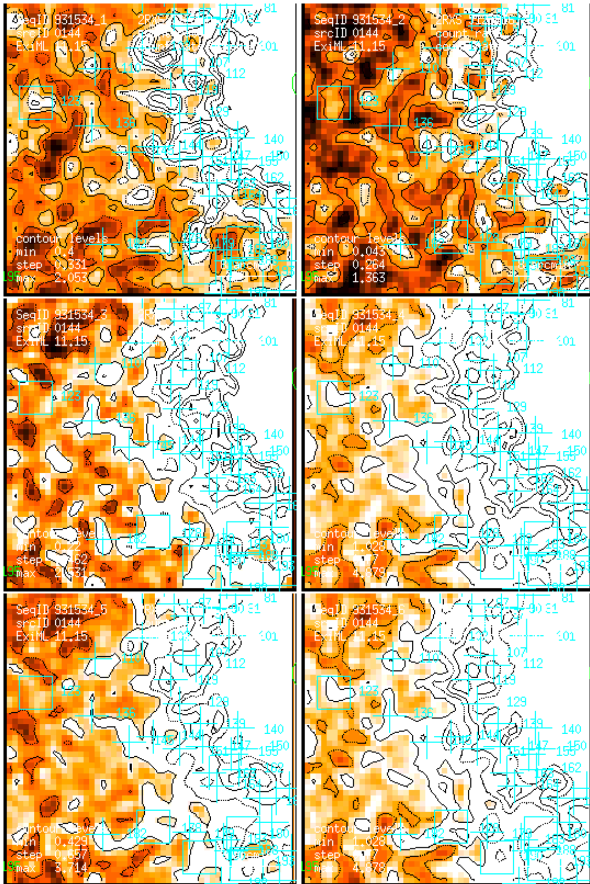
Figure 144: RASS 931534: detection 0144: band rate images, Gaussian filter: (1) PSPC channels 11 – 41, (2) 52 – 90, (3) 91 – 201, (4) 11 – 235, (5) 52 – 201, (6) 11 – 201. Broad band rates in counts/ks. Band rate contour levels in counts/ks/arcmin 2 .
