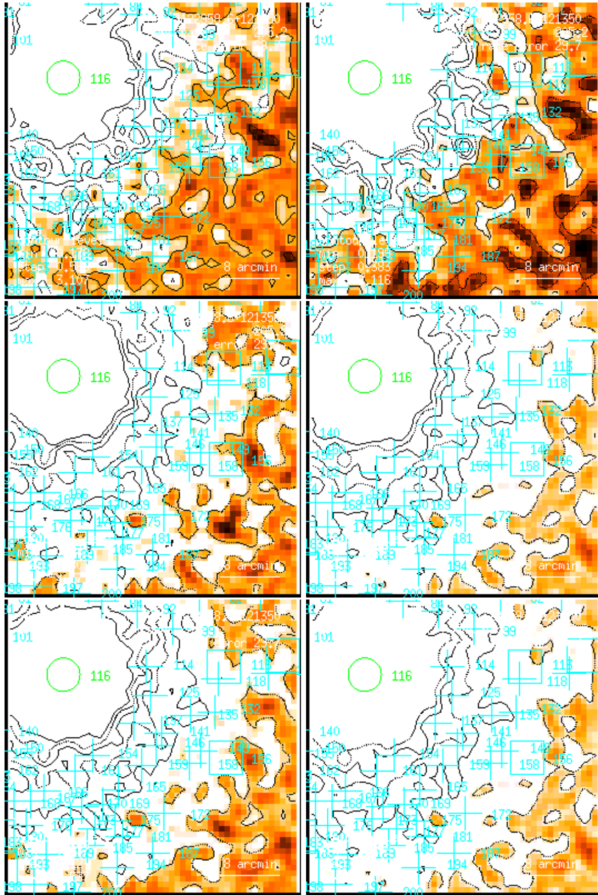
Figure 146: RASS 931534: detection 0146: band rate images, Gaussian filter: (1) PSPC channels 11 – 41, (2) 52 – 90, (3) 91 – 201, (4) 11 – 235, (5) 52 – 201, (6) 11 – 201. Broad band rates in counts/ks. Band rate contour levels in counts/ks/arcmin 2 .
