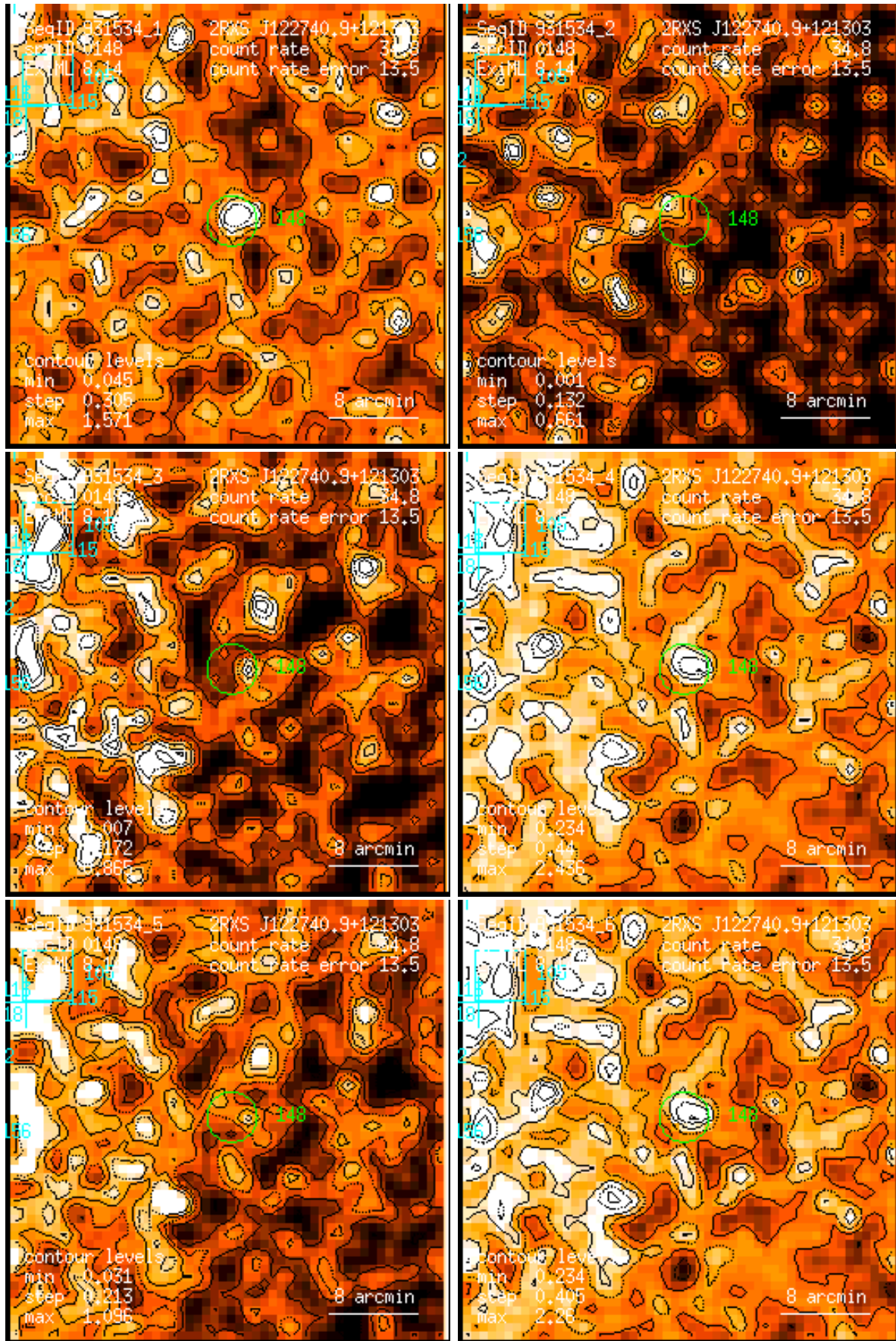
Figure 148: RASS 931534: detection 0148: band rate images, Gaussian filter: (1) PSPC channels 11 – 41, (2) 52 – 90, (3) 91 – 201, (4) 11 – 235, (5) 52 – 201, (6) 11 – 201. Broad band rates in counts/ks. Band rate contour levels in counts/ks/arcmin 2 .
