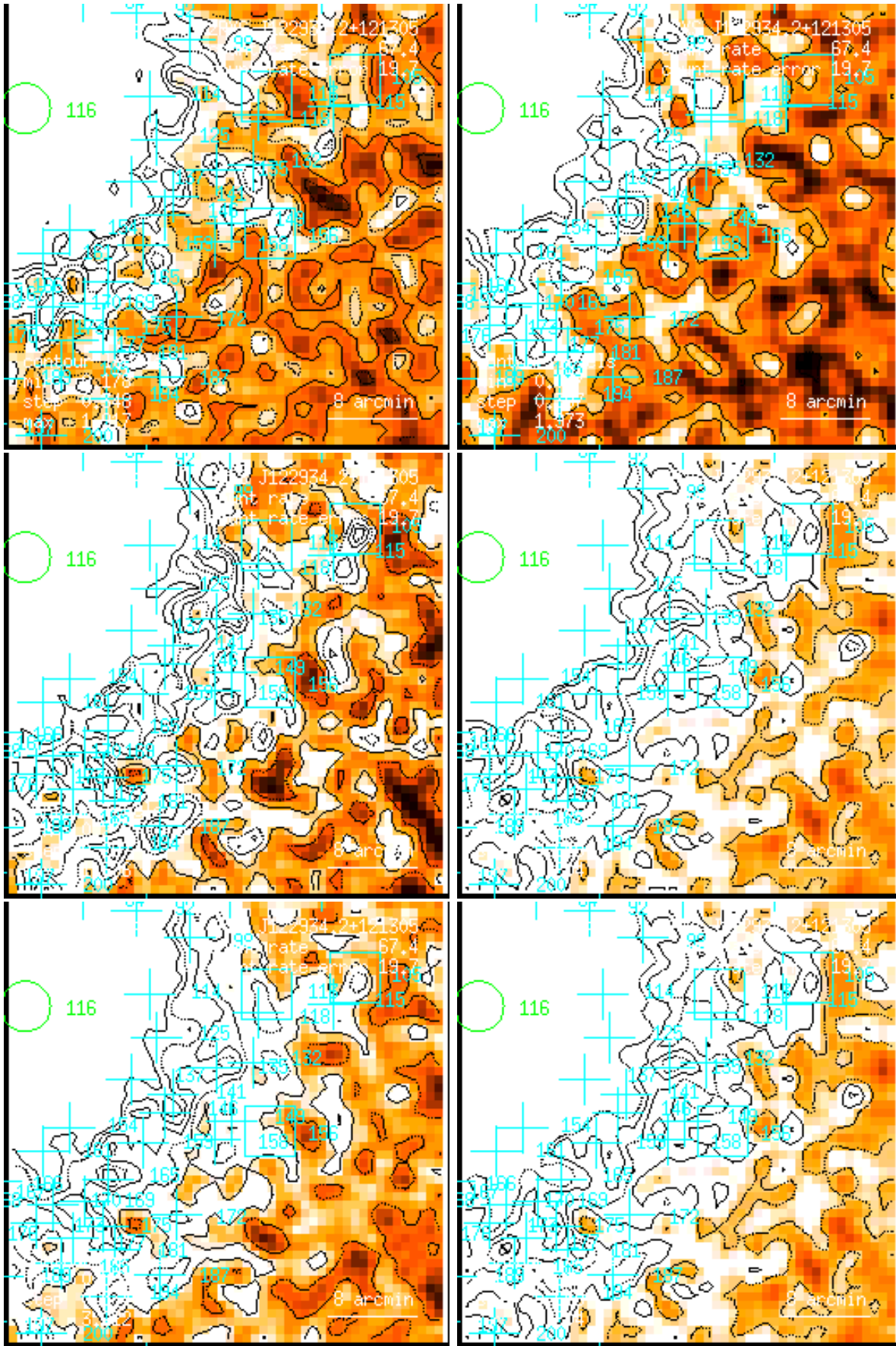
Figure 149: RASS 931534: detection 0149: band rate images, Gaussian filter: (1) PSPC channels 11 – 41, (2) 52 – 90, (3) 91 – 201, (4) 11 – 235, (5) 52 – 201, (6) 11 – 201. Broad band rates in counts/ks. Band rate contour levels in counts/ks/arcmin 2 .
