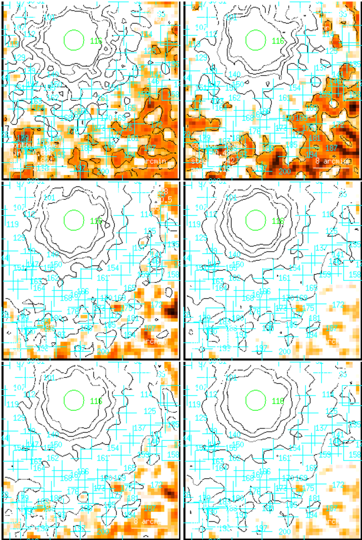
Figure 154: RASS 931534: detection 0154: band rate images, Gaussian filter: (1) PSPC channels 11 – 41, (2) 52 – 90, (3) 91 – 201, (4) 11 – 235, (5) 52 – 201, (6) 11 – 201. Broad band rates in counts/ks. Band rate contour levels in counts/ks/arcmin 2 .
