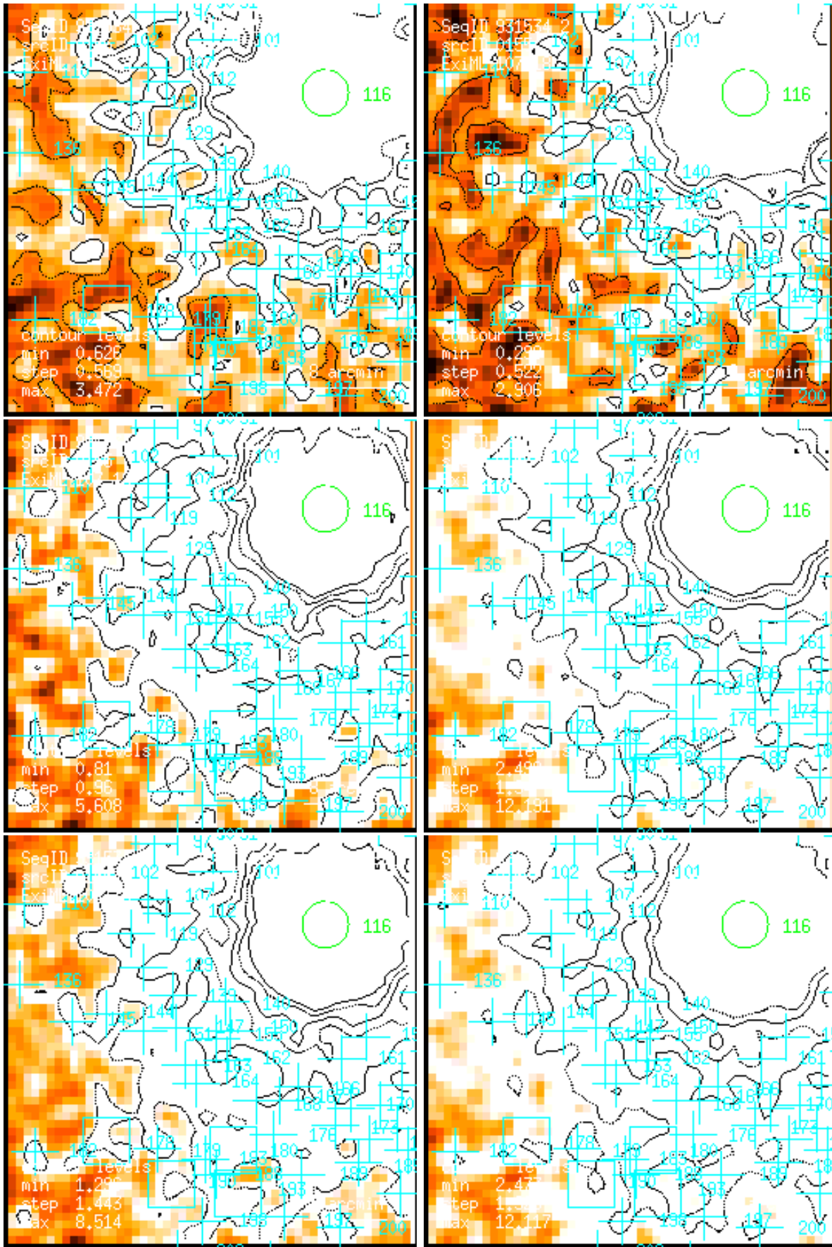
Figure 155: RASS 931534: detection 0155: band rate images, Gaussian filter: (1) PSPC channels 11 – 41, (2) 52 – 90, (3) 91 – 201, (4) 11 – 235, (5) 52 – 201, (6) 11 – 201. Broad band rates in counts/ks. Band rate contour levels in counts/ks/arcmin 2 .
