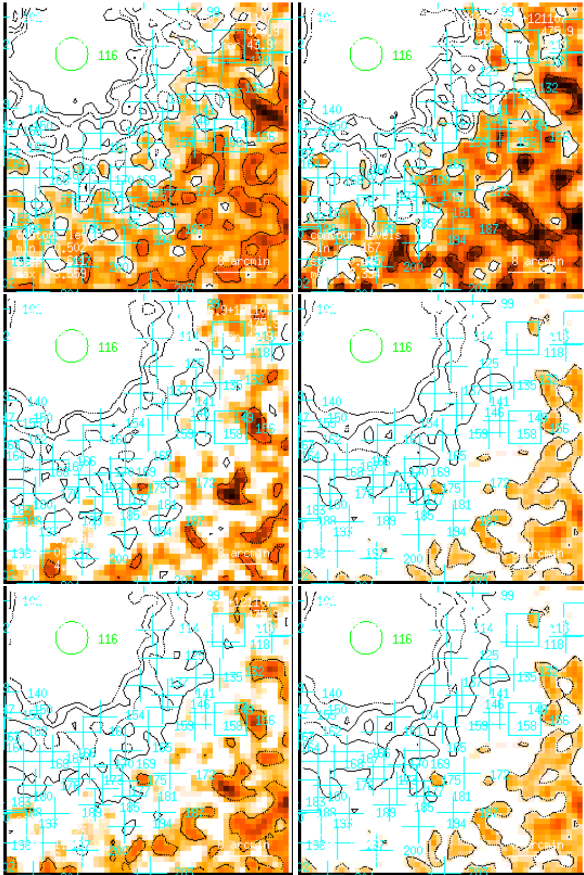
Figure 159: RASS 931534: detection 0159: band rate images, Gaussian filter: (1) PSPC channels 11 – 41, (2) 52 – 90, (3) 91 – 201, (4) 11 – 235, (5) 52 – 201, (6) 11 – 201. Broad band rates in counts/ks. Band rate contour levels in counts/ks/arcmin 2 .
