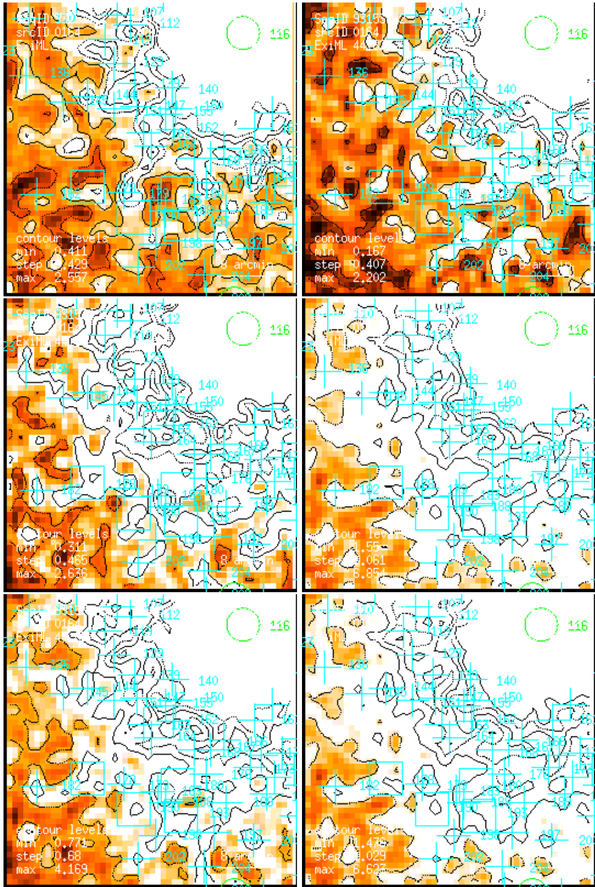
Figure 164: RASS 931534: detection 0164: band rate images, Gaussian filter: (1) PSPC channels 11 – 41, (2) 52 – 90, (3) 91 – 201, (4) 11 – 235, (5) 52 – 201, (6) 11 – 201. Broad band rates in counts/ks. Band rate contour levels in counts/ks/arcmin 2 .
