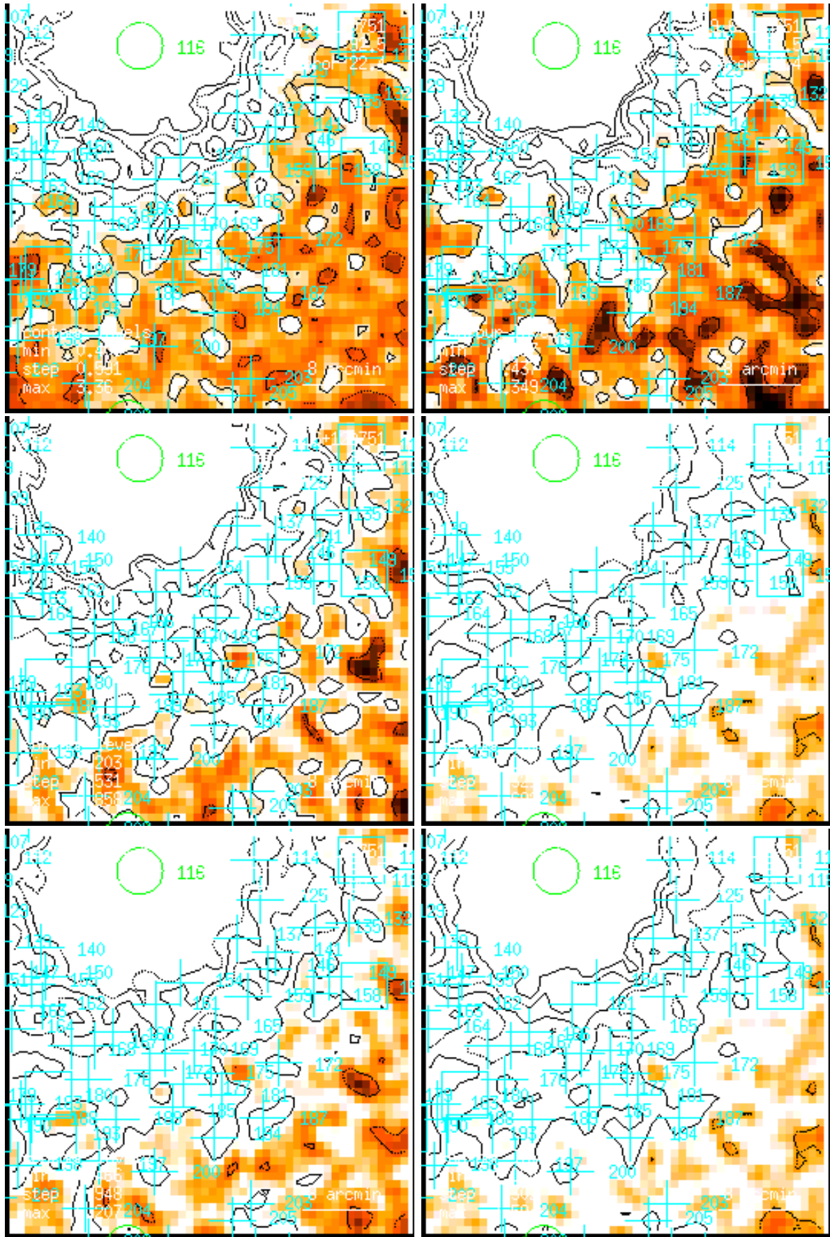
Figure 165: RASS 931534: detection 0165: band rate images, Gaussian filter: (1) PSPC channels 11 – 41, (2) 52 – 90, (3) 91 – 201, (4) 11 – 235, (5) 52 – 201, (6) 11 – 201. Broad band rates in counts/ks. Band rate contour levels in counts/ks/arcmin 2 .
