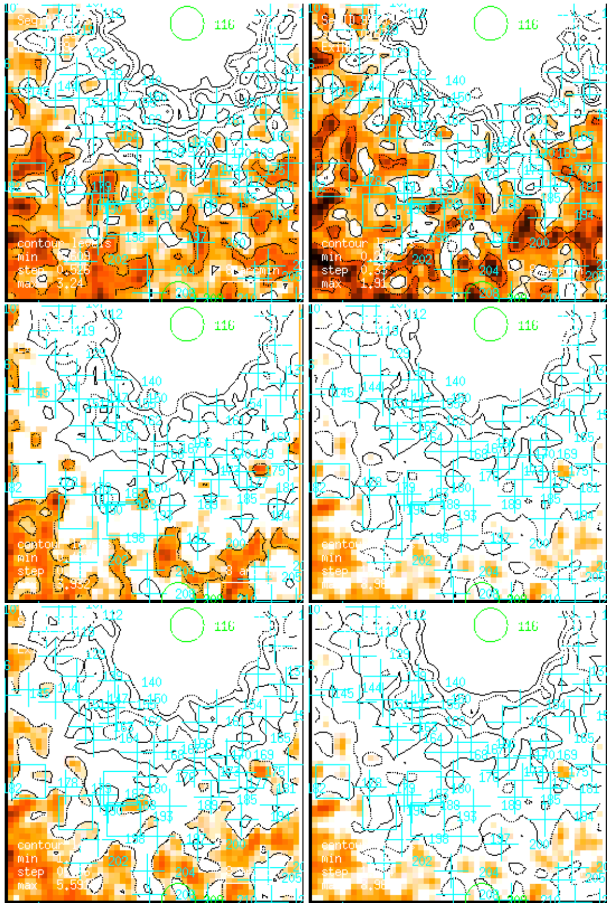
Figure 167: RASS 931534: detection 0167: band rate images, Gaussian filter: (1) PSPC channels 11 – 41, (2) 52 – 90, (3) 91 – 201, (4) 11 – 235, (5) 52 – 201, (6) 11 – 201. Broad band rates in counts/ks. Band rate contour levels in counts/ks/arcmin 2 .
