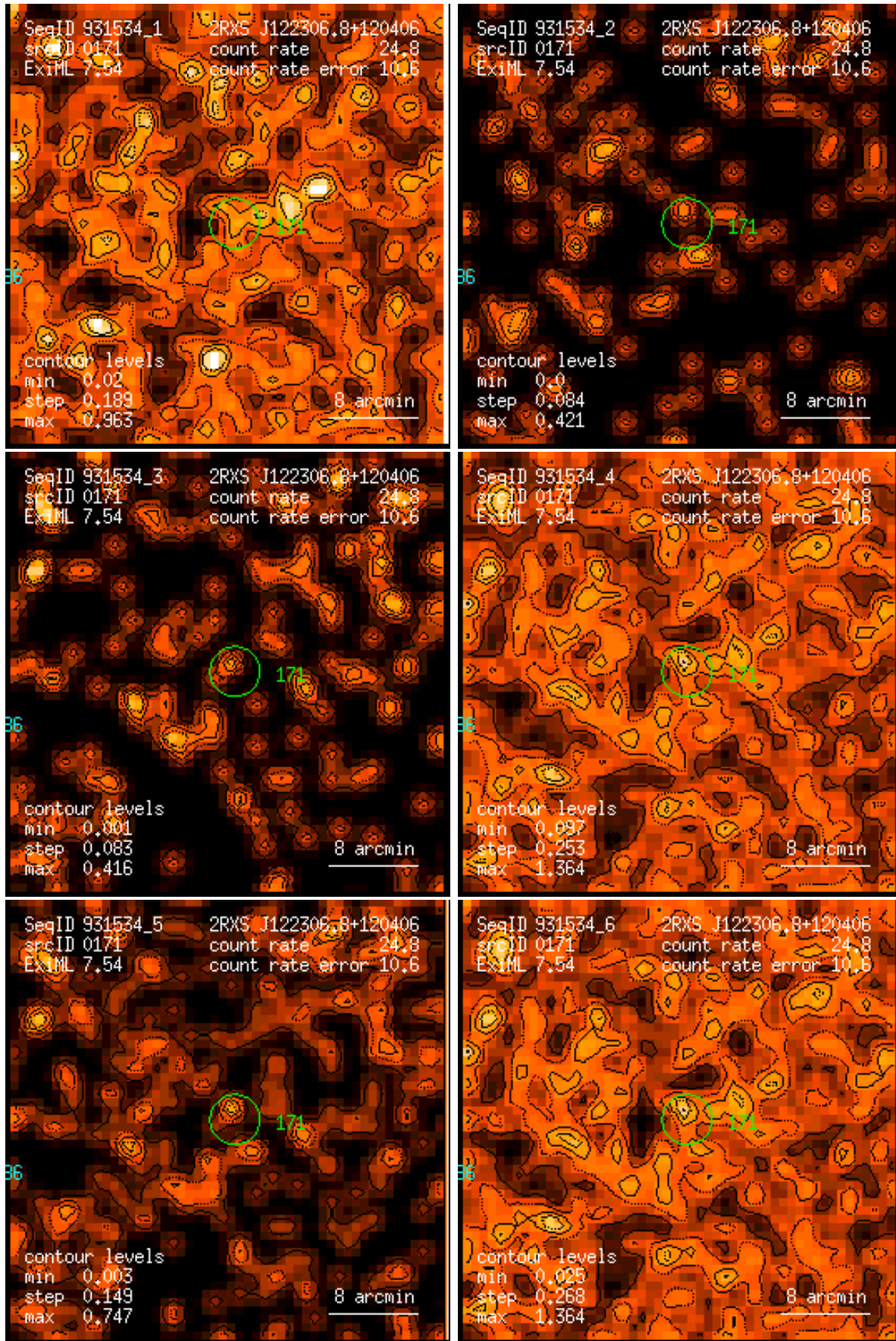
Figure 171: RASS 931534: detection 0171: band rate images, Gaussian filter: (1) PSPC channels 11 – 41, (2) 52 – 90, (3) 91 – 201, (4) 11 – 235, (5) 52 – 201, (6) 11 – 201. Broad band rates in counts/ks. Band rate contour levels in counts/ks/arcmin 2 .
