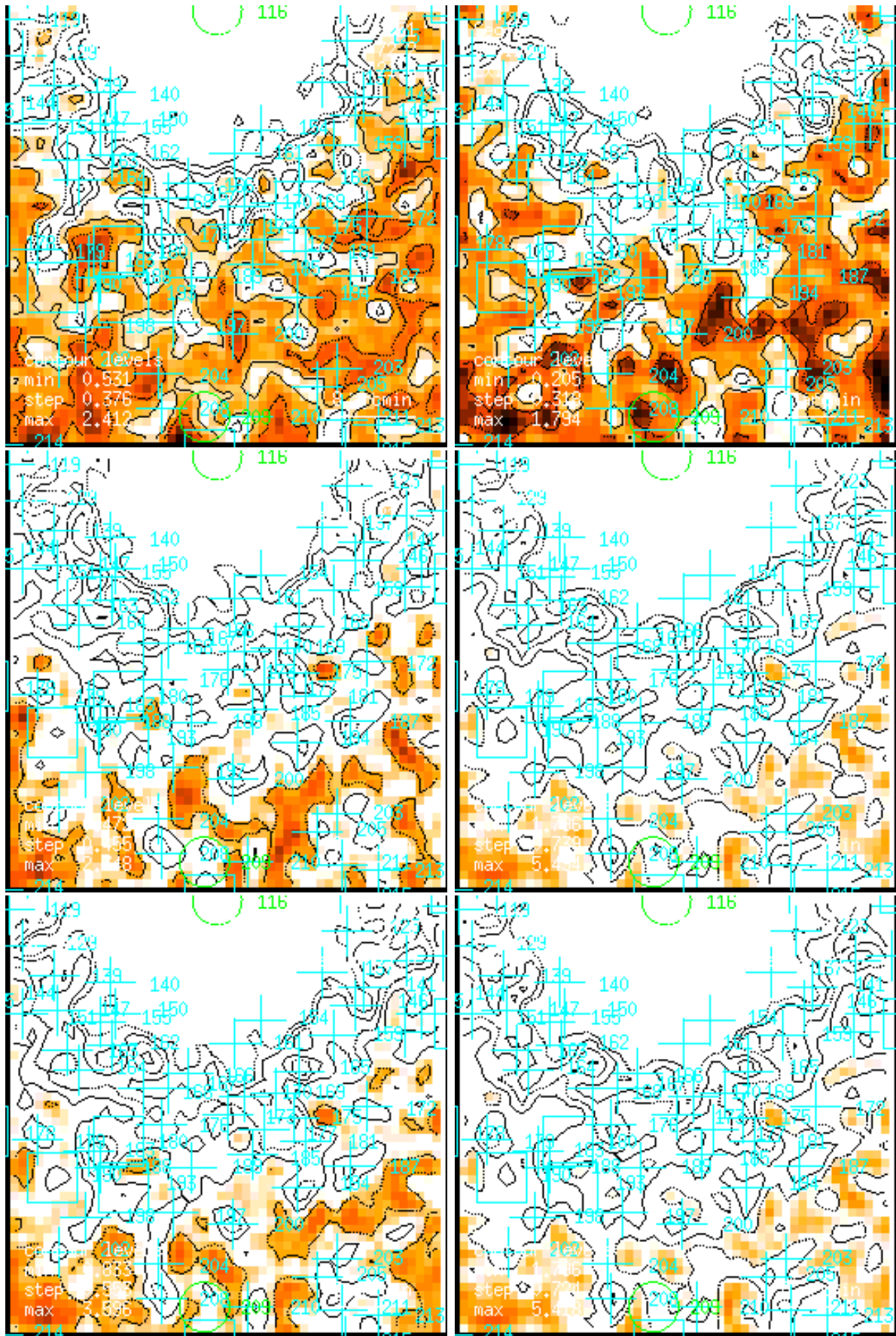
Figure 173: RASS 931534: detection 0173: band rate images, Gaussian filter: (1) PSPC channels 11 – 41, (2) 52 – 90, (3) 91 – 201, (4) 11 – 235, (5) 52 – 201, (6) 11 – 201. Broad band rates in counts/ks. Band rate contour levels in counts/ks/arcmin 2 .
