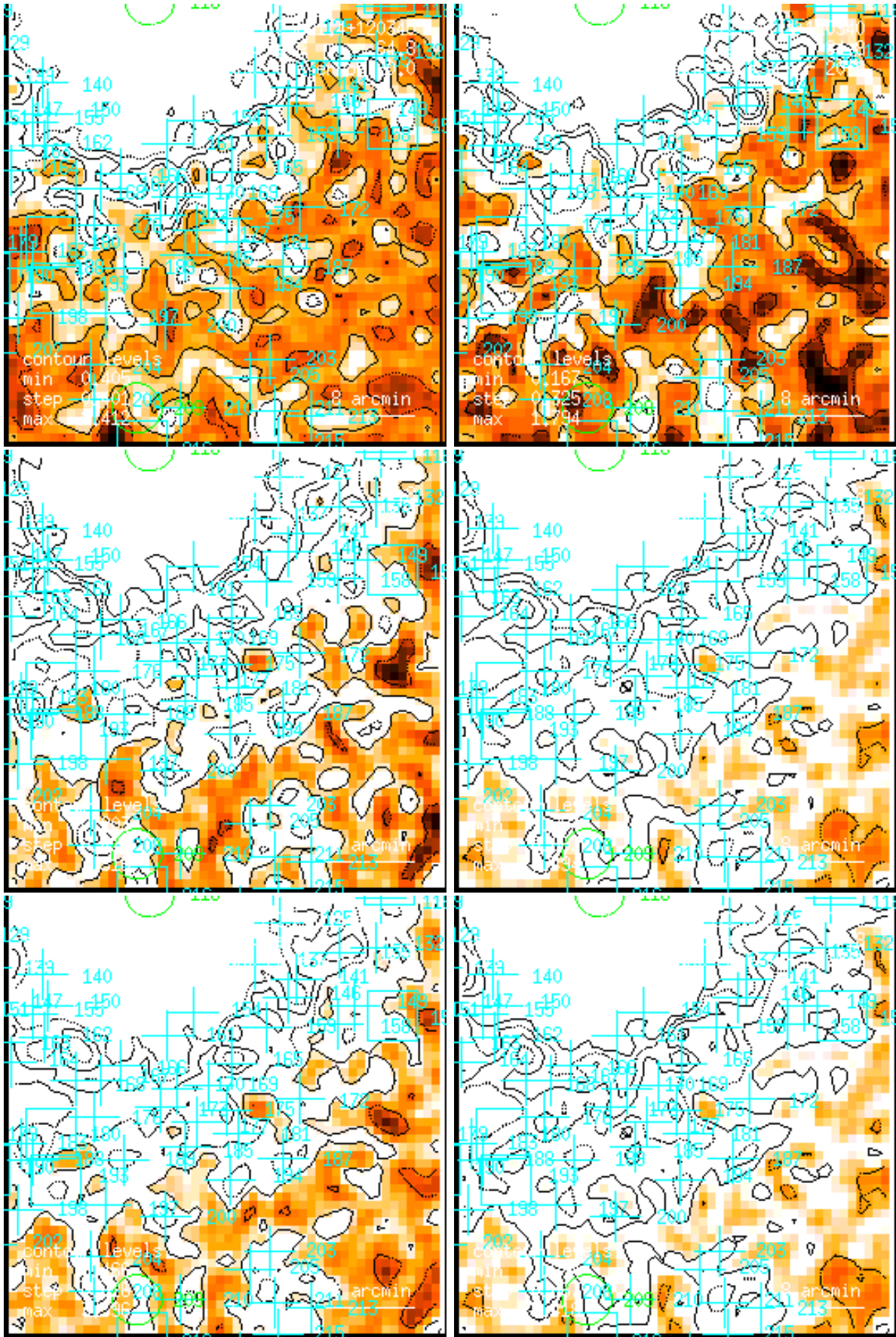
Figure 175: RASS 931534: detection 0175: band rate images, Gaussian filter: (1) PSPC channels 11 – 41, (2) 52 – 90, (3) 91 – 201, (4) 11 – 235, (5) 52 – 201, (6) 11 – 201. Broad band rates in counts/ks. Band rate contour levels in counts/ks/arcmin 2 .
