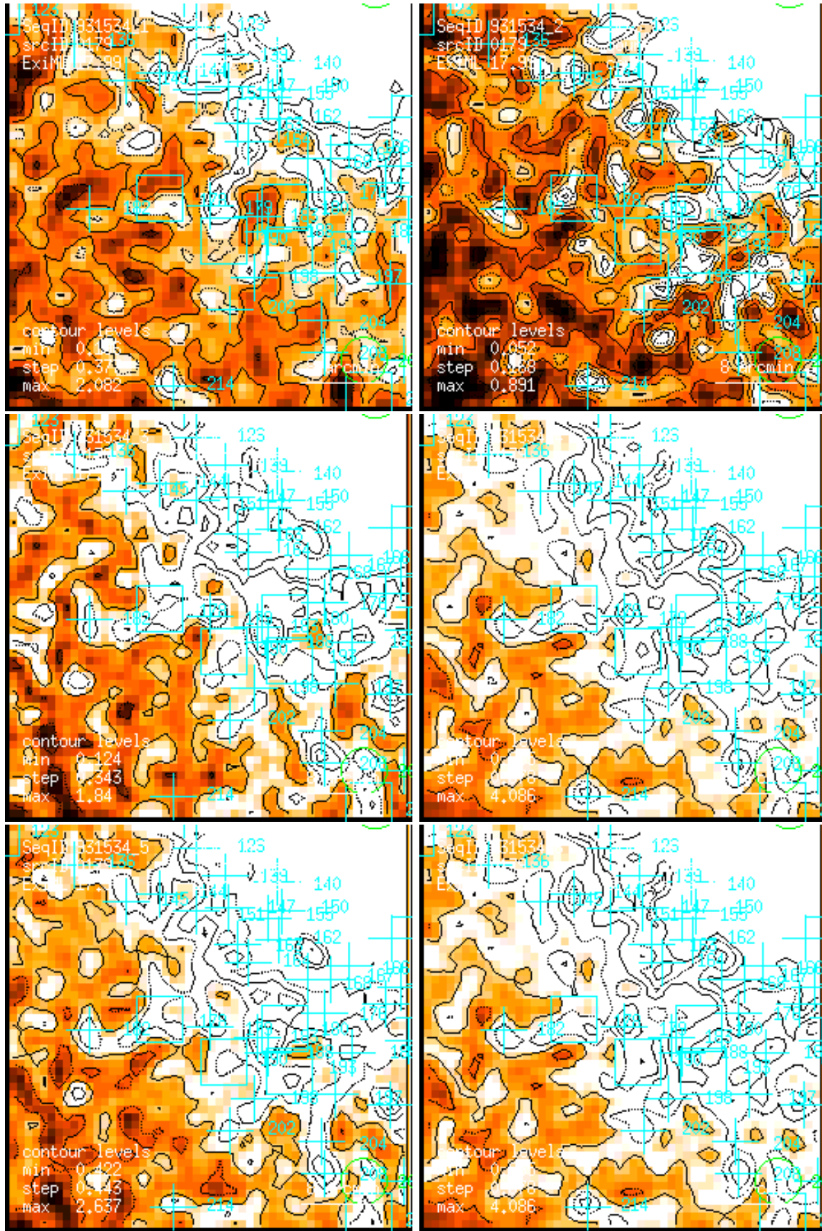
Figure 179: RASS 931534: detection 0179: band rate images, Gaussian filter: (1) PSPC channels 11 – 41, (2) 52 – 90, (3) 91 – 201, (4) 11 – 235, (5) 52 – 201, (6) 11 – 201. Broad band rates in counts/ks. Band rate contour levels in counts/ks/arcmin 2 .
