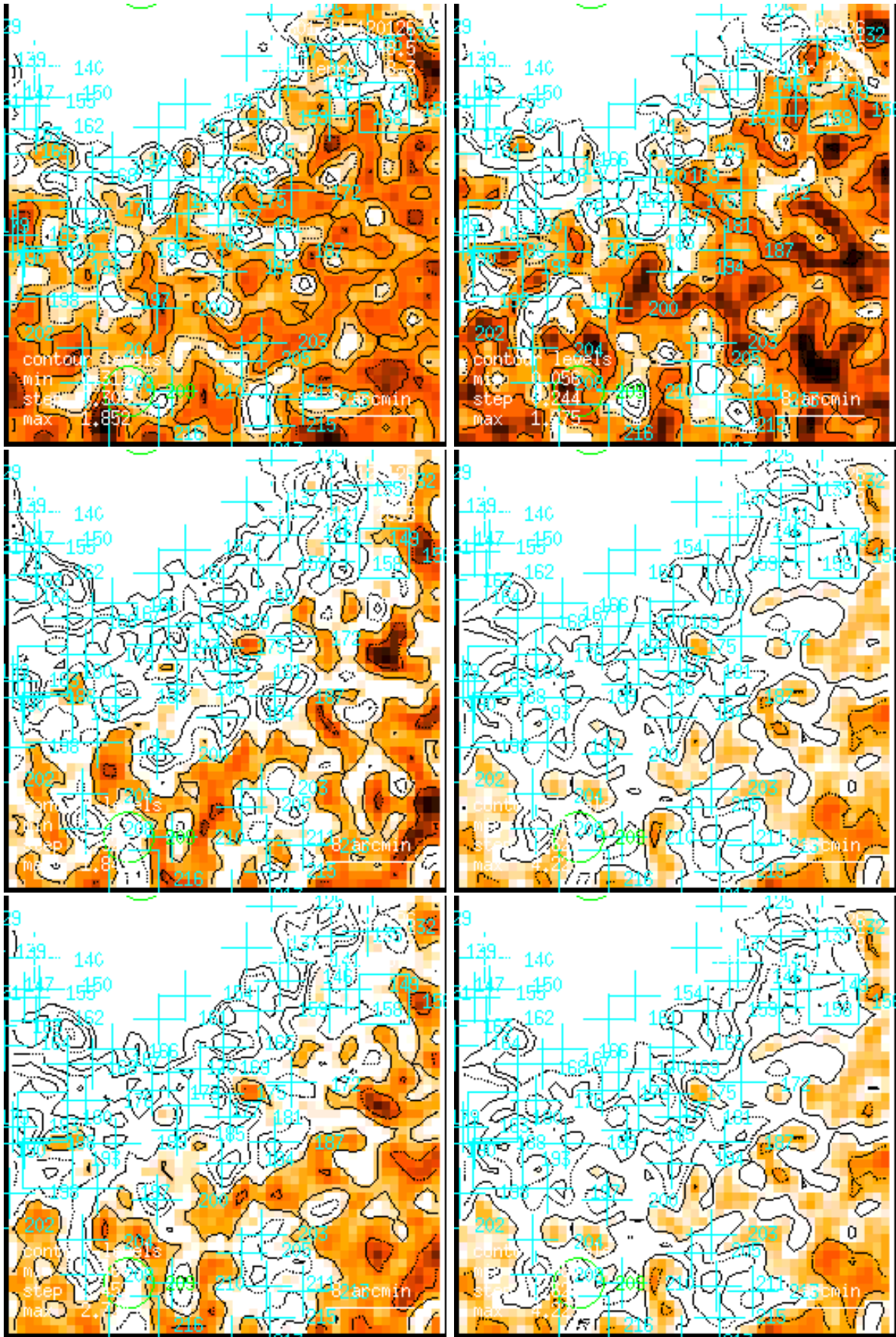
Figure 181: RASS 931534: detection 0181: band rate images, Gaussian filter: (1) PSPC channels 11 – 41, (2) 52 – 90, (3) 91 – 201, (4) 11 – 235, (5) 52 – 201, (6) 11 – 201. Broad band rates in counts/ks. Band rate contour levels in counts/ks/arcmin 2 .
