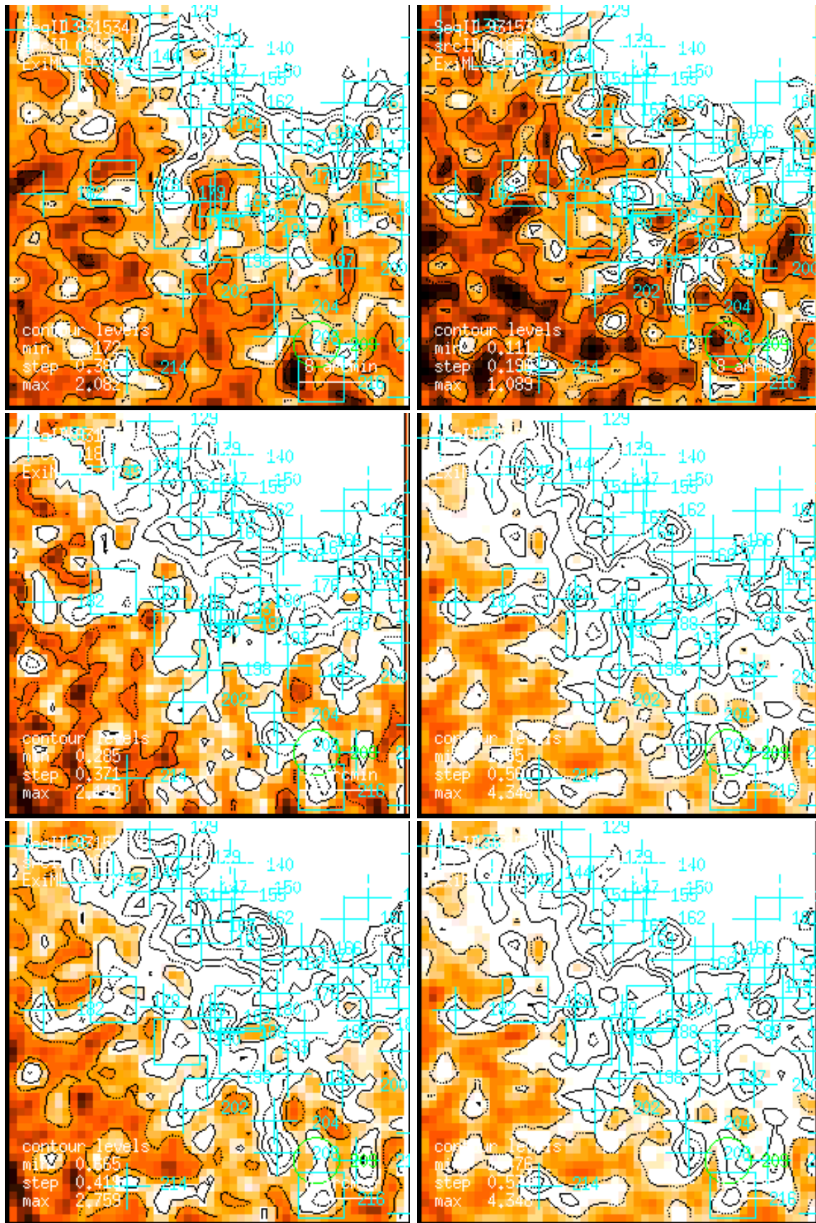
Figure 183: RASS 931534: detection 0183: band rate images, Gaussian filter: (1) PSPC channels 11 – 41, (2) 52 – 90, (3) 91 – 201, (4) 11 – 235, (5) 52 – 201, (6) 11 – 201. Broad band rates in counts/ks. Band rate contour levels in counts/ks/arcmin 2 .
