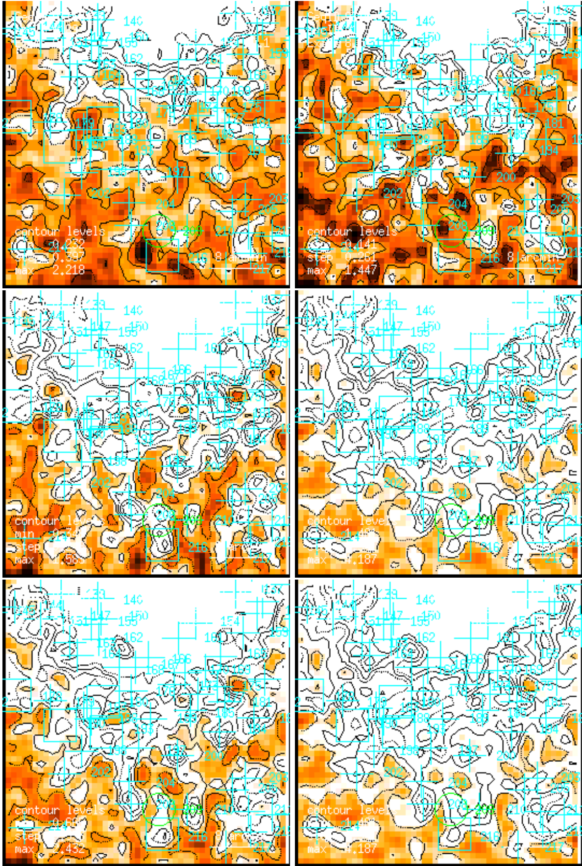
Figure 189: RASS 931534: detection 0189: band rate images, Gaussian filter: (1) PSPC channels 11 – 41, (2) 52 – 90, (3) 91 – 201, (4) 11 – 235, (5) 52 – 201, (6) 11 – 201. Broad band rates in counts/ks. Band rate contour levels in counts/ks/arcmin 2 .
