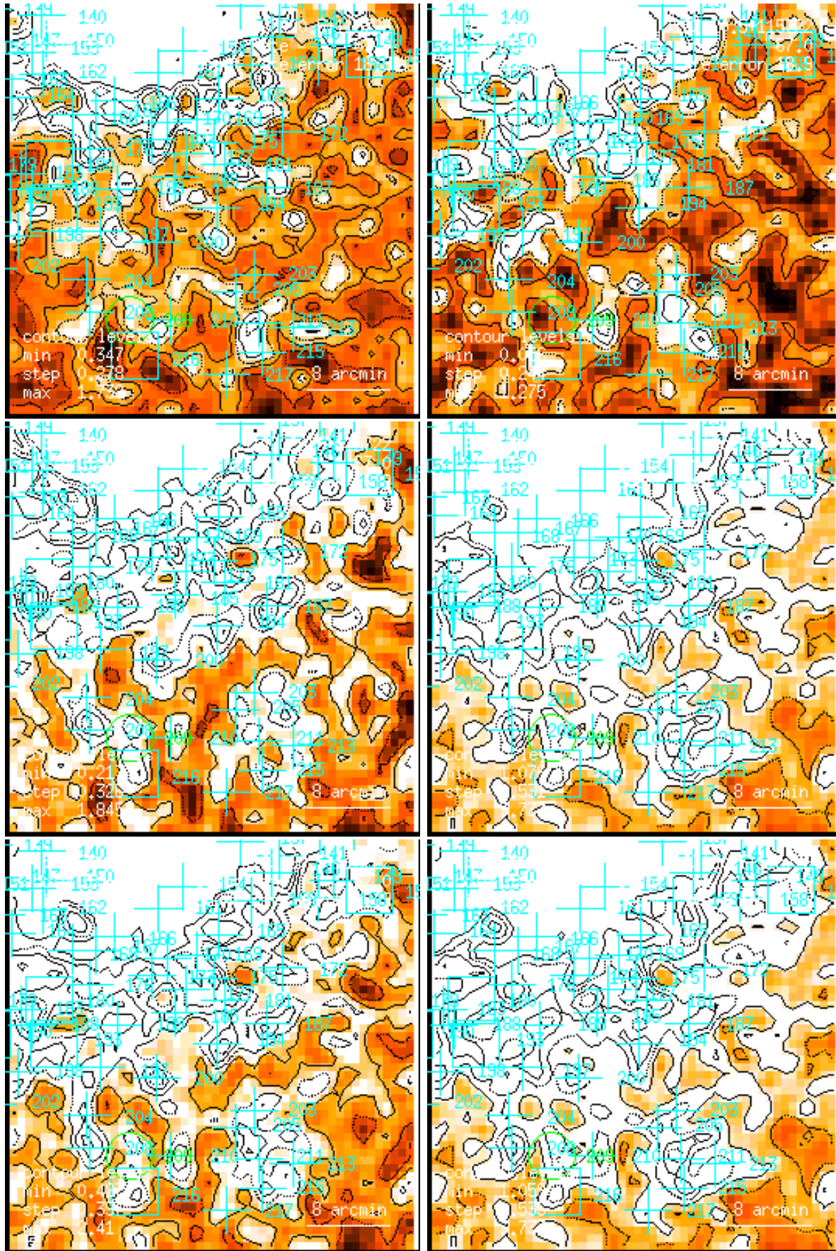
Figure 194: RASS 931534: detection 0194: band rate images, Gaussian filter: (1) PSPC channels 11 – 41, (2) 52 – 90, (3) 91 – 201, (4) 11 – 235, (5) 52 – 201, (6) 11 – 201. Broad band rates in counts/ks. Band rate contour levels in counts/ks/arcmin 2 .
