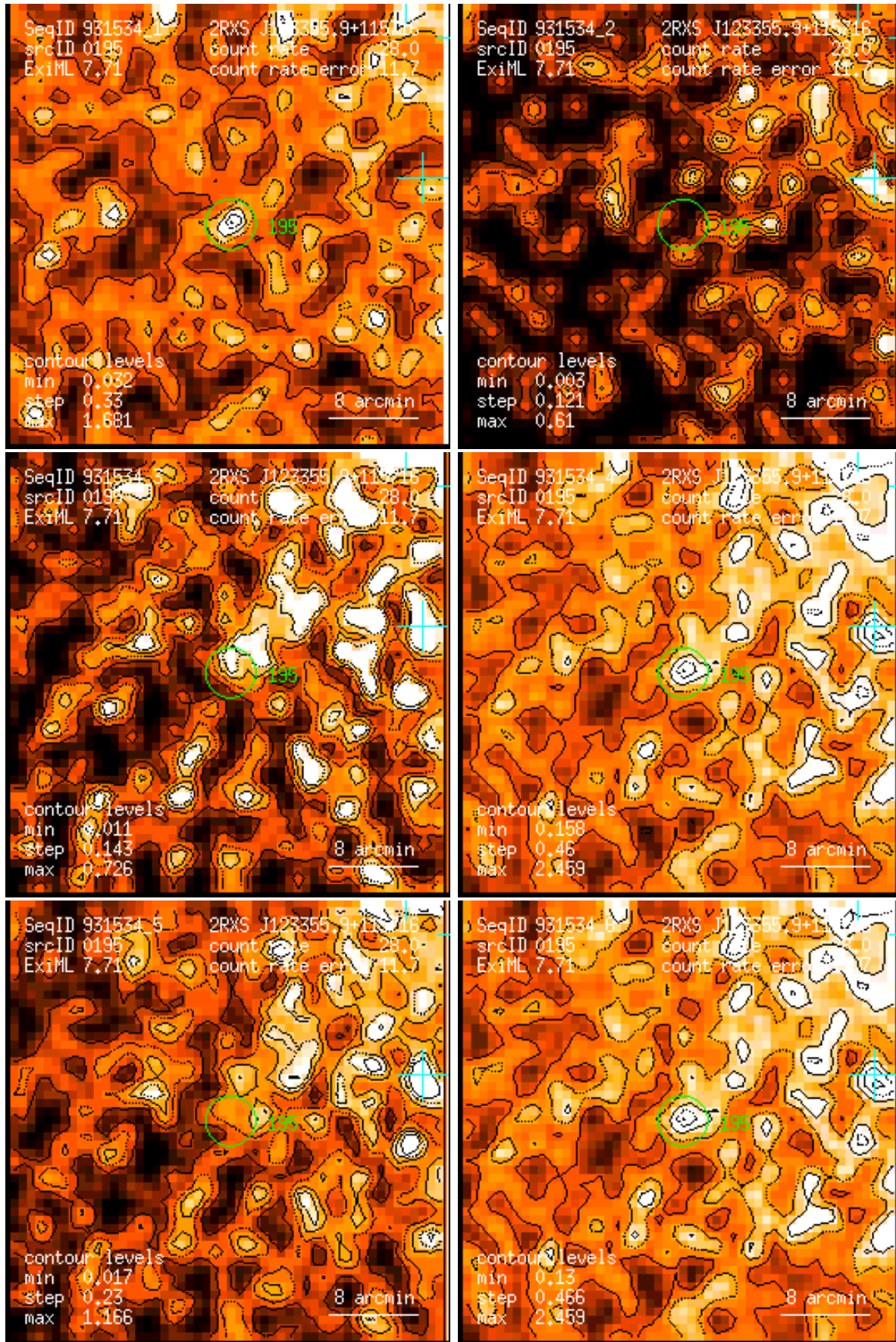
Figure 195: RASS 931534: detection 0195: band rate images, Gaussian filter: (1) PSPC channels 11 – 41, (2) 52 – 90, (3) 91 – 201, (4) 11 – 235, (5) 52 – 201, (6) 11 – 201. Broad band rates in counts/ks. Band rate contour levels in counts/ks/arcmin 2 .
