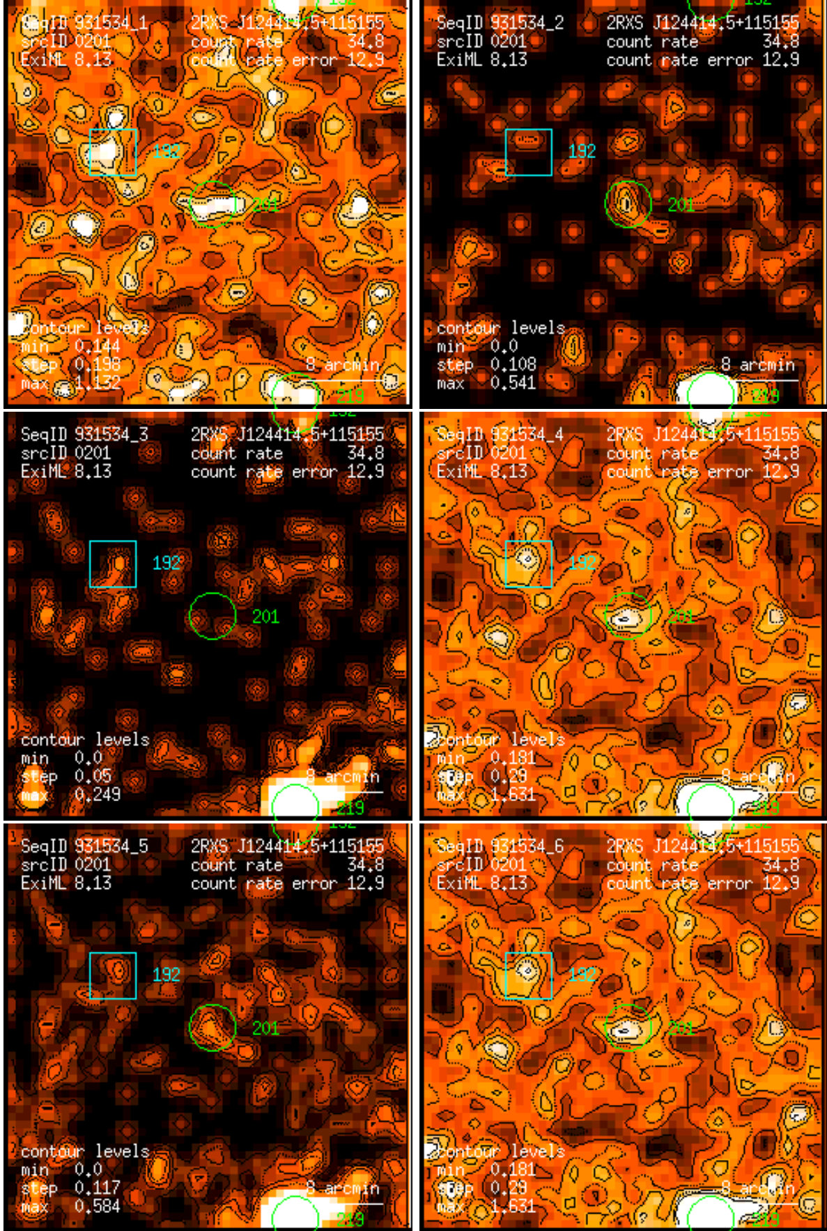
Figure 201: RASS 931534: detection 0201: band rate images, Gaussian filter: (1) PSPC channels 11 – 41, (2) 52 – 90, (3) 91 – 201, (4) 11 – 235, (5) 52 – 201, (6) 11 – 201. Broad band rates in counts/ks. Band rate contour levels in counts/ks/arcmin 2 .
