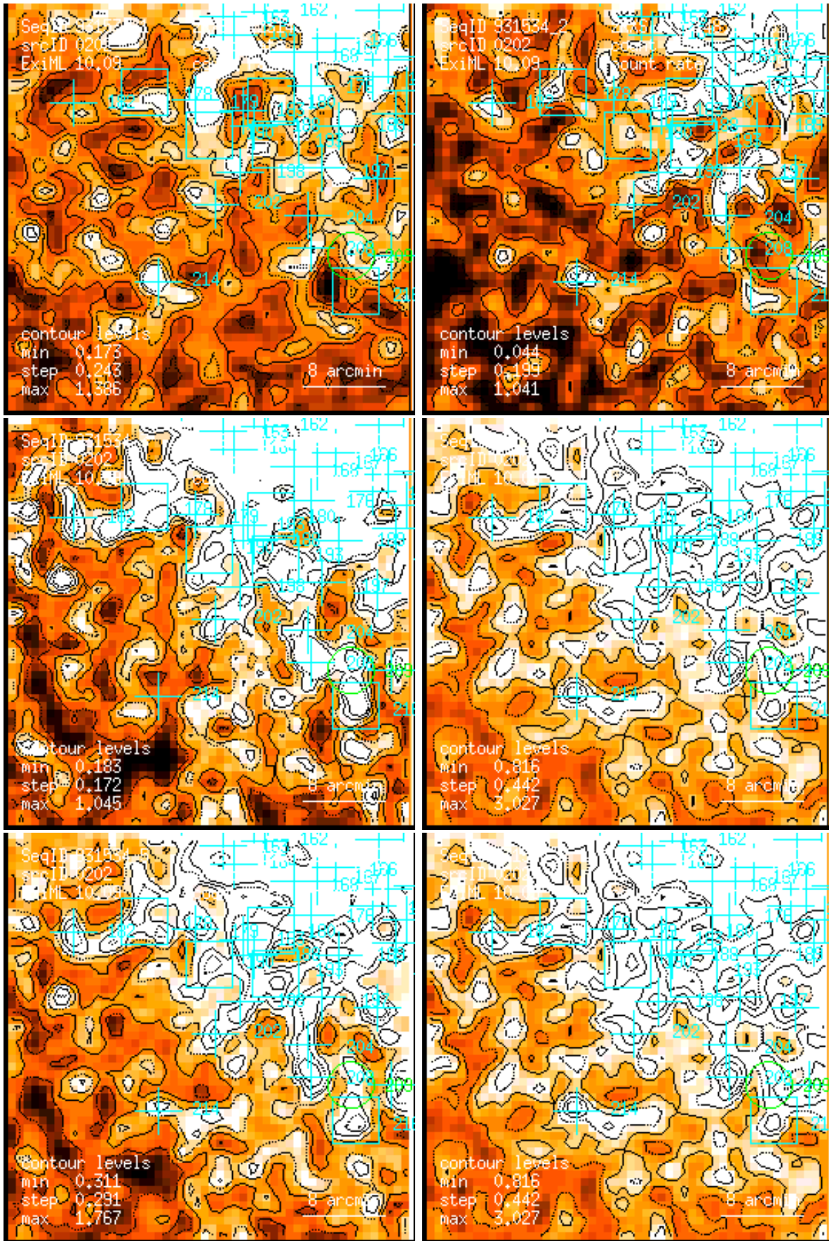
Figure 202: RASS 931534: detection 0202: band rate images, Gaussian filter: (1) PSPC channels 11 – 41, (2) 52 – 90, (3) 91 – 201, (4) 11 – 235, (5) 52 – 201, (6) 11 – 201. Broad band rates in counts/ks. Band rate contour levels in counts/ks/arcmin 2 .
