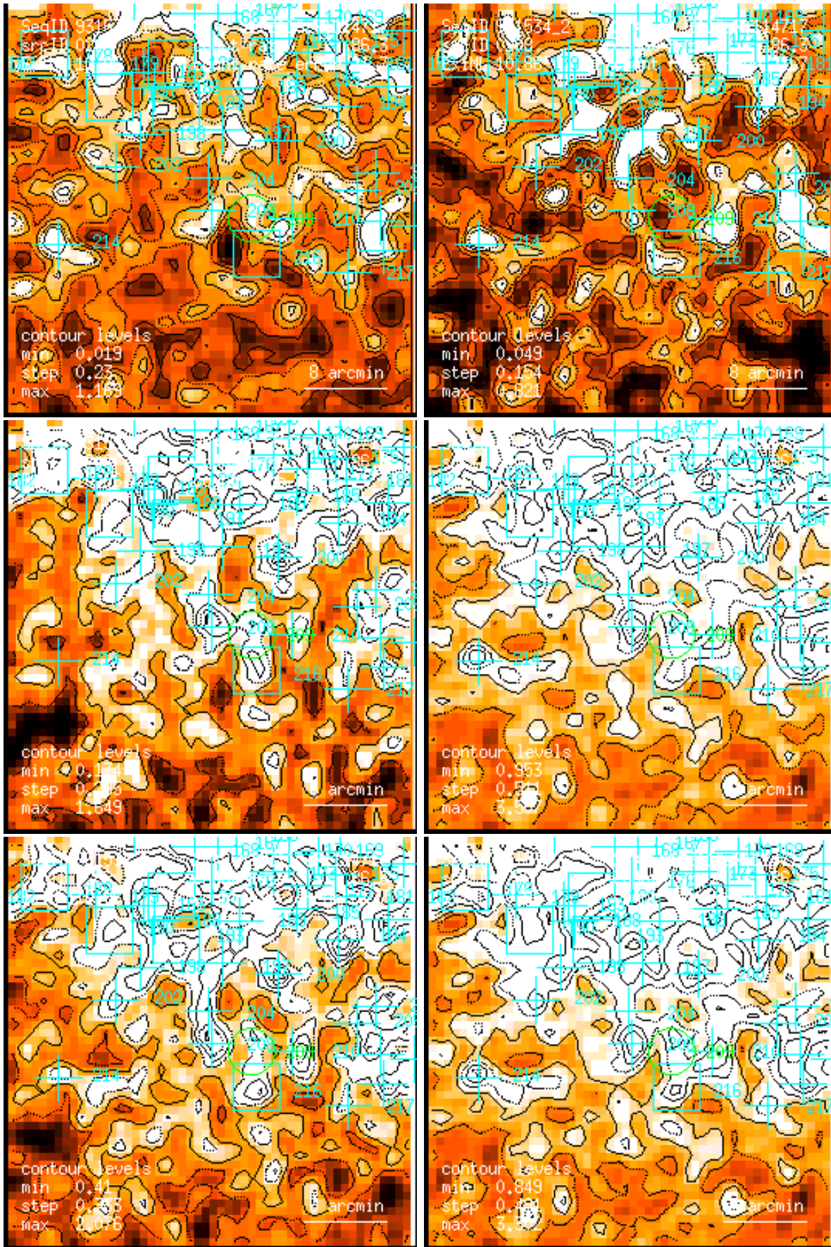
Figure 208: RASS 931534: detection 0208: band rate images, Gaussian filter: (1) PSPC channels 11 – 41, (2) 52 – 90, (3) 91 – 201, (4) 11 – 235, (5) 52 – 201, (6) 11 – 201. Broad band rates in counts/ks. Band rate contour levels in counts/ks/arcmin 2 .
