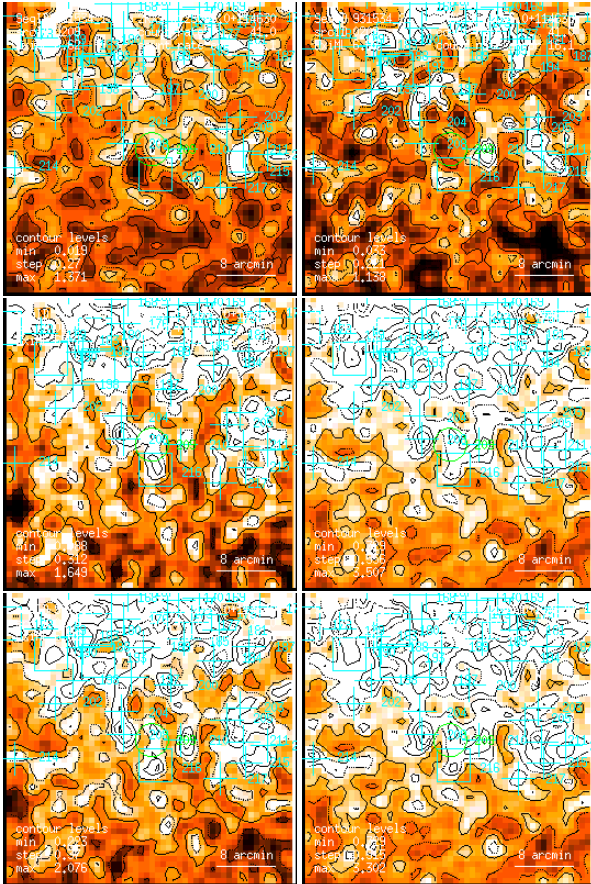
Figure 209: RASS 931534: detection 0209: band rate images, Gaussian filter: (1) PSPC channels 11 – 41, (2) 52 – 90, (3) 91 – 201, (4) 11 – 235, (5) 52 – 201, (6) 11 – 201. Broad band rates in counts/ks. Band rate contour levels in counts/ks/arcmin 2 .
