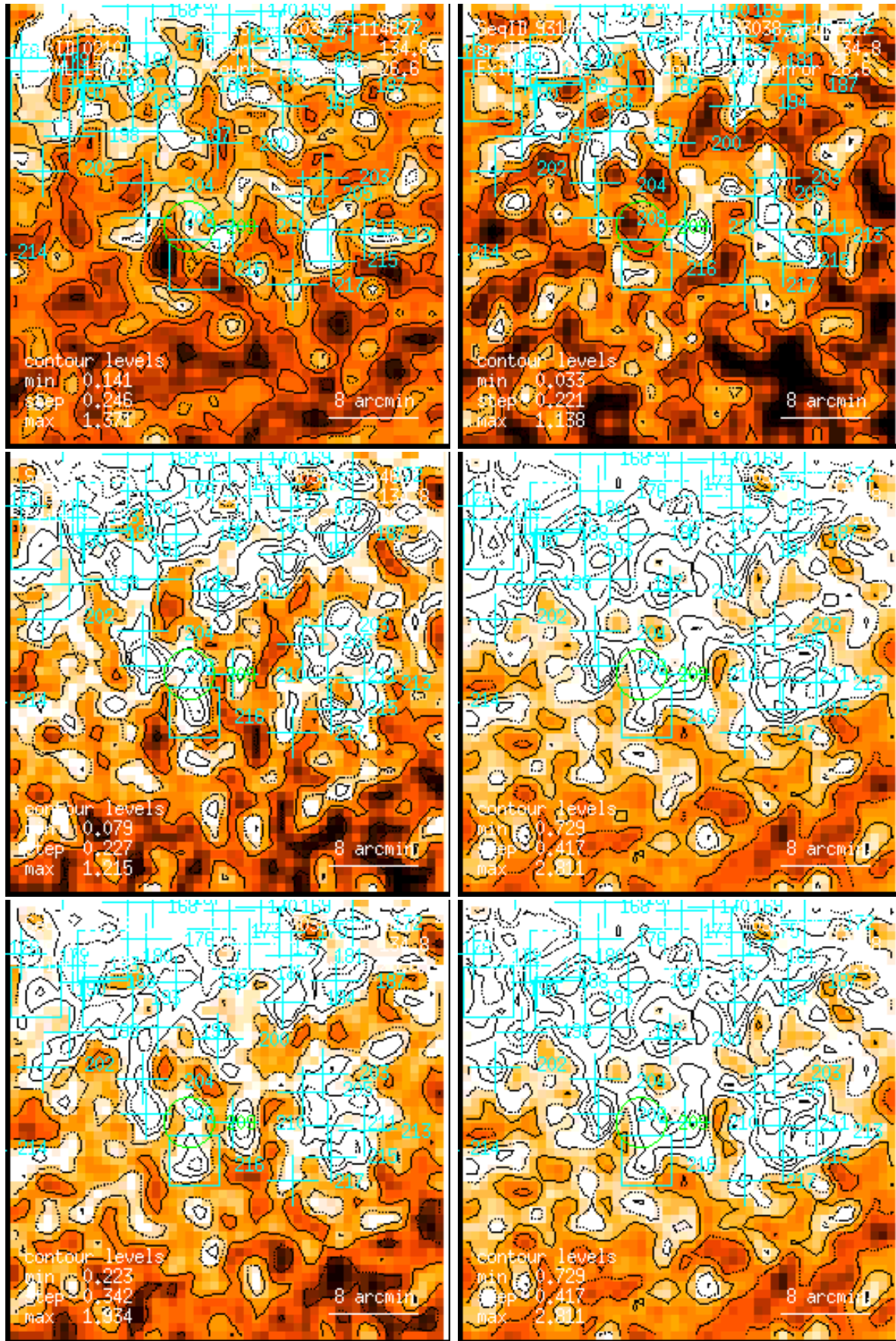
Figure 210: RASS 931534: detection 0210: band rate images, Gaussian filter: (1) PSPC channels 11 – 41, (2) 52 – 90, (3) 91 – 201, (4) 11 – 235, (5) 52 – 201, (6) 11 – 201. Broad band rates in counts/ks. Band rate contour levels in counts/ks/arcmin 2 .
