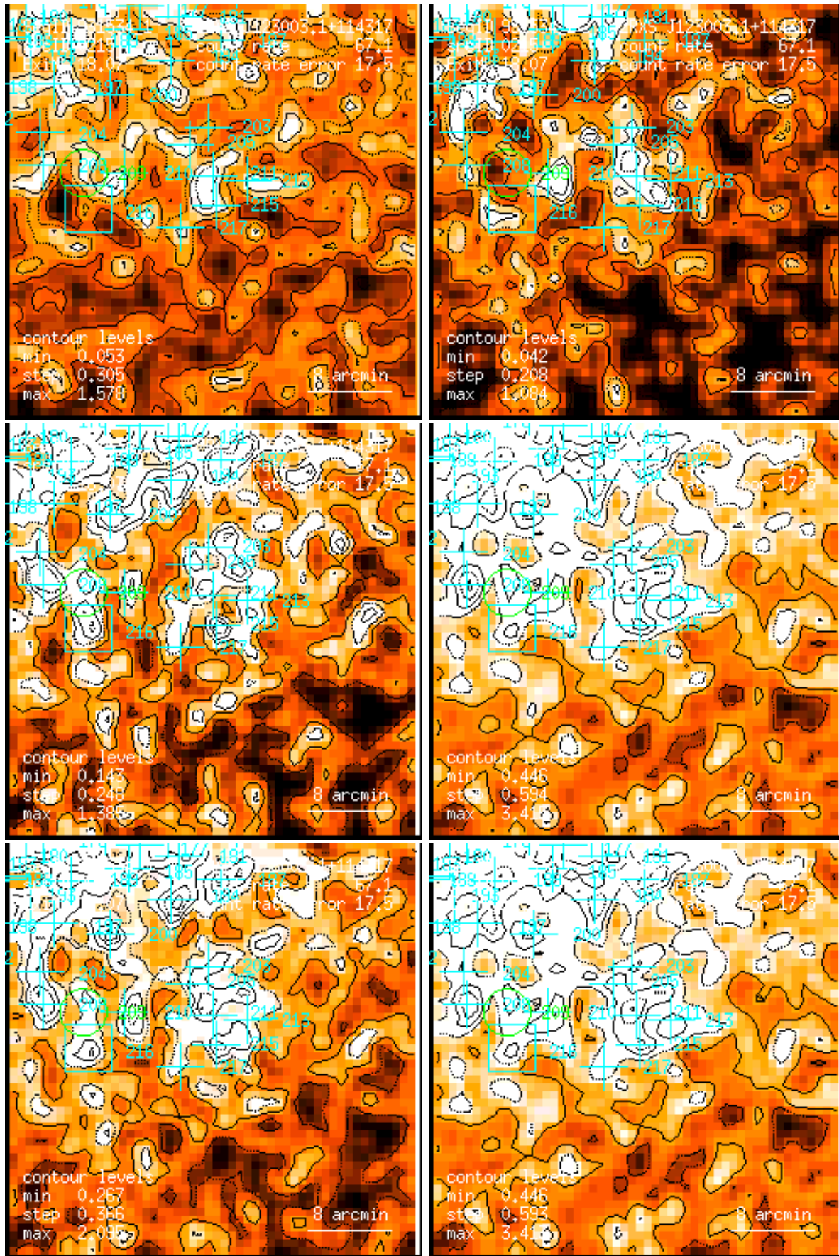
Figure 215: RASS 931534: detection 0215: band rate images, Gaussian filter: (1) PSPC channels 11 – 41, (2) 52 – 90, (3) 91 – 201, (4) 11 – 235, (5) 52 – 201, (6) 11 – 201. Broad band rates in counts/ks. Band rate contour levels in counts/ks/arcmin 2 .
