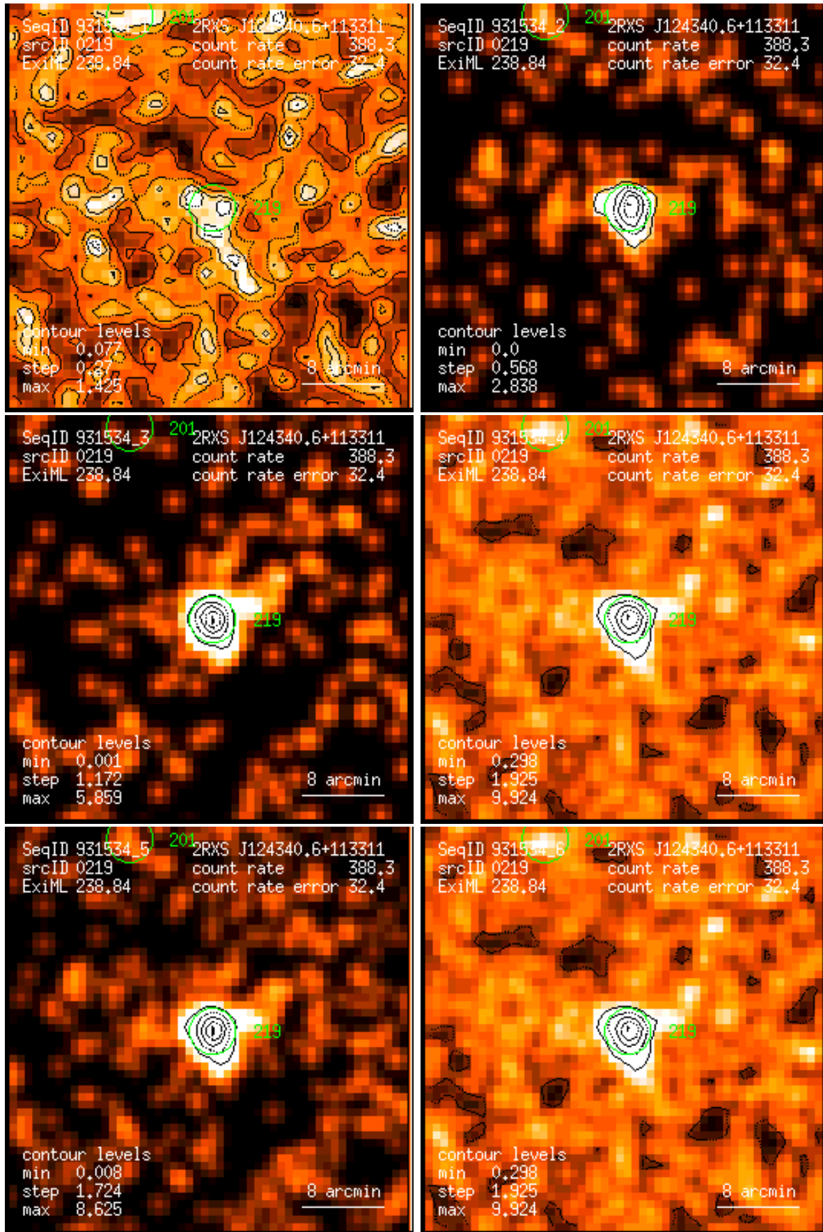
Figure 219: RASS 931534: detection 0219: band rate images, Gaussian filter: (1) PSPC channels 11 – 41, (2) 52 – 90, (3) 91 – 201, (4) 11 – 235, (5) 52 – 201, (6) 11 – 201. Broad band rates in counts/ks. Band rate contour levels in counts/ks/arcmin 2 .
