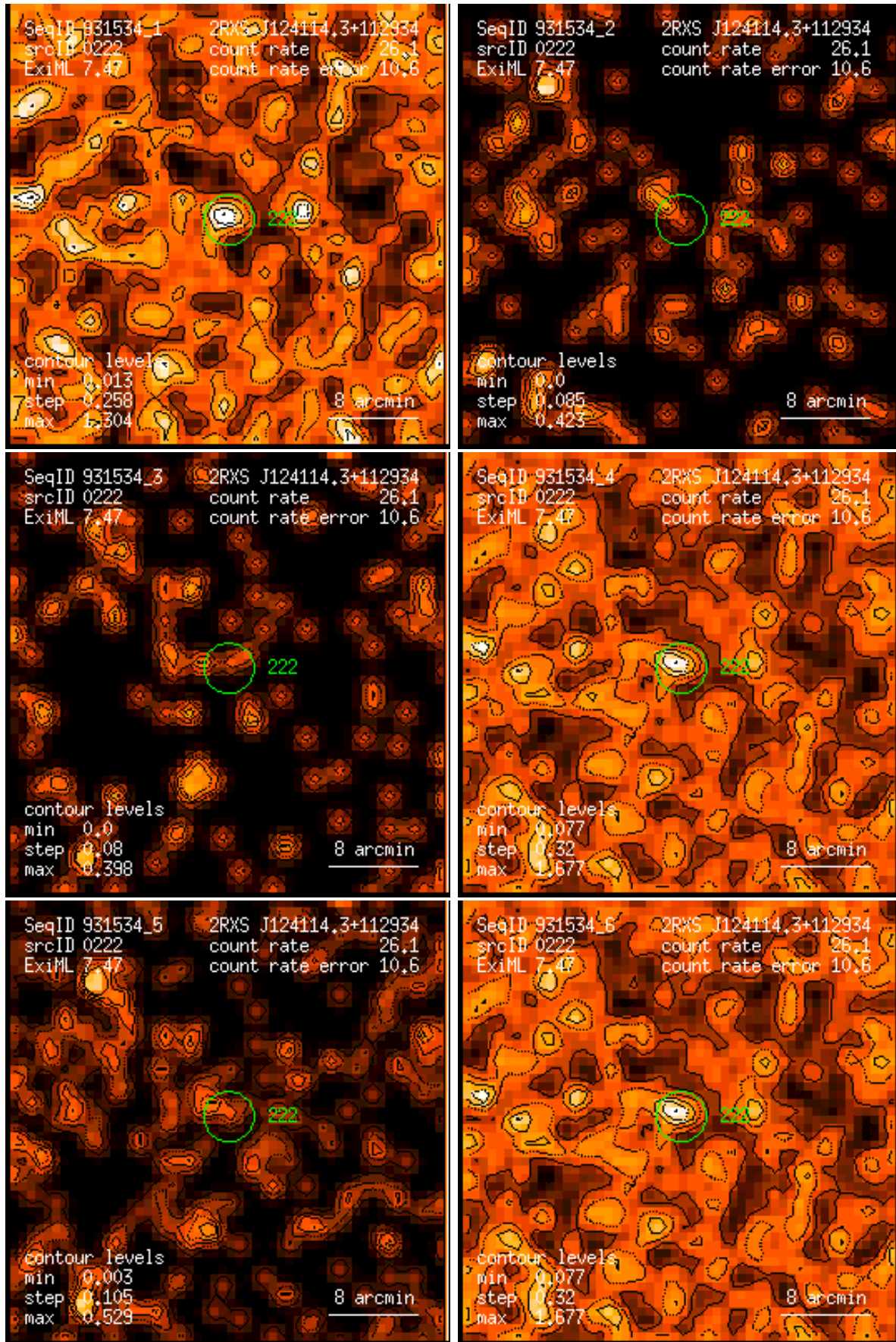
Figure 222: RASS 931534: detection 0222: band rate images, Gaussian filter: (1) PSPC channels 11 – 41, (2) 52 – 90, (3) 91 – 201, (4) 11 – 235, (5) 52 – 201, (6) 11 – 201. Broad band rates in counts/ks. Band rate contour levels in counts/ks/arcmin 2 .
