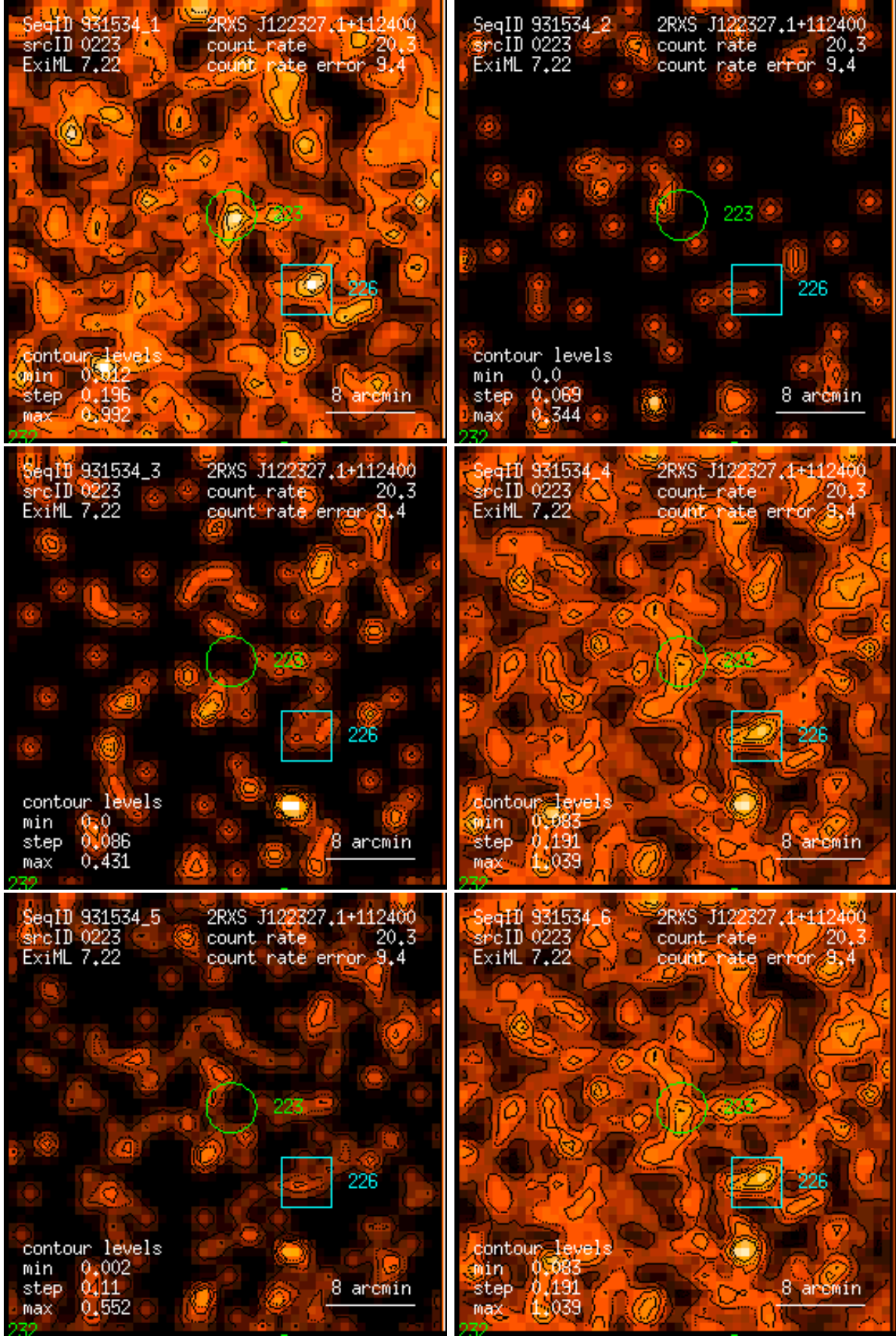
Figure 223: RASS 931534: detection 0223: band rate images, Gaussian filter: (1) PSPC channels 11 – 41, (2) 52 – 90, (3) 91 – 201, (4) 11 – 235, (5) 52 – 201, (6) 11 – 201. Broad band rates in counts/ks. Band rate contour levels in counts/ks/arcmin 2 .
