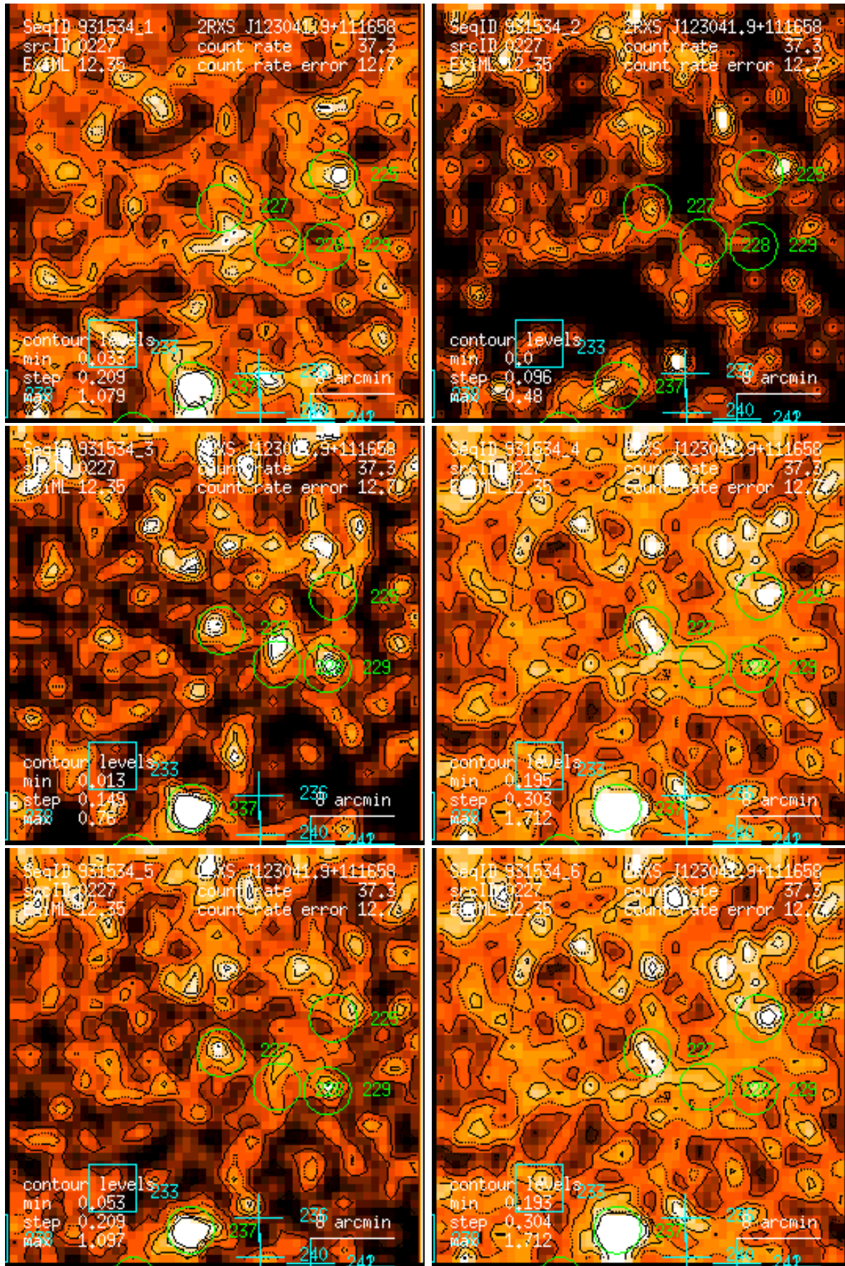
Figure 227: RASS 931534: detection 0227: band rate images, Gaussian filter: (1) PSPC channels 11 – 41, (2) 52 – 90, (3) 91 – 201, (4) 11 – 235, (5) 52 – 201, (6) 11 – 201. Broad band rates in counts/ks. Band rate contour levels in counts/ks/arcmin 2 .
