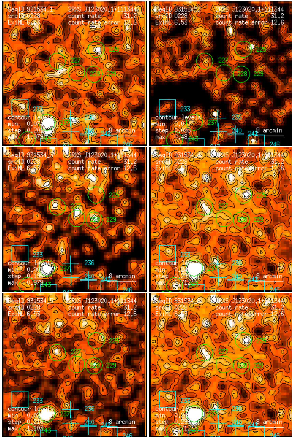
Figure 228: RASS 931534: detection 0228: band rate images, Gaussian filter: (1) PSPC channels 11 – 41, (2) 52 – 90, (3) 91 – 201, (4) 11 – 235, (5) 52 – 201, (6) 11 – 201. Broad band rates in counts/ks. Band rate contour levels in counts/ks/arcmin 2 .
