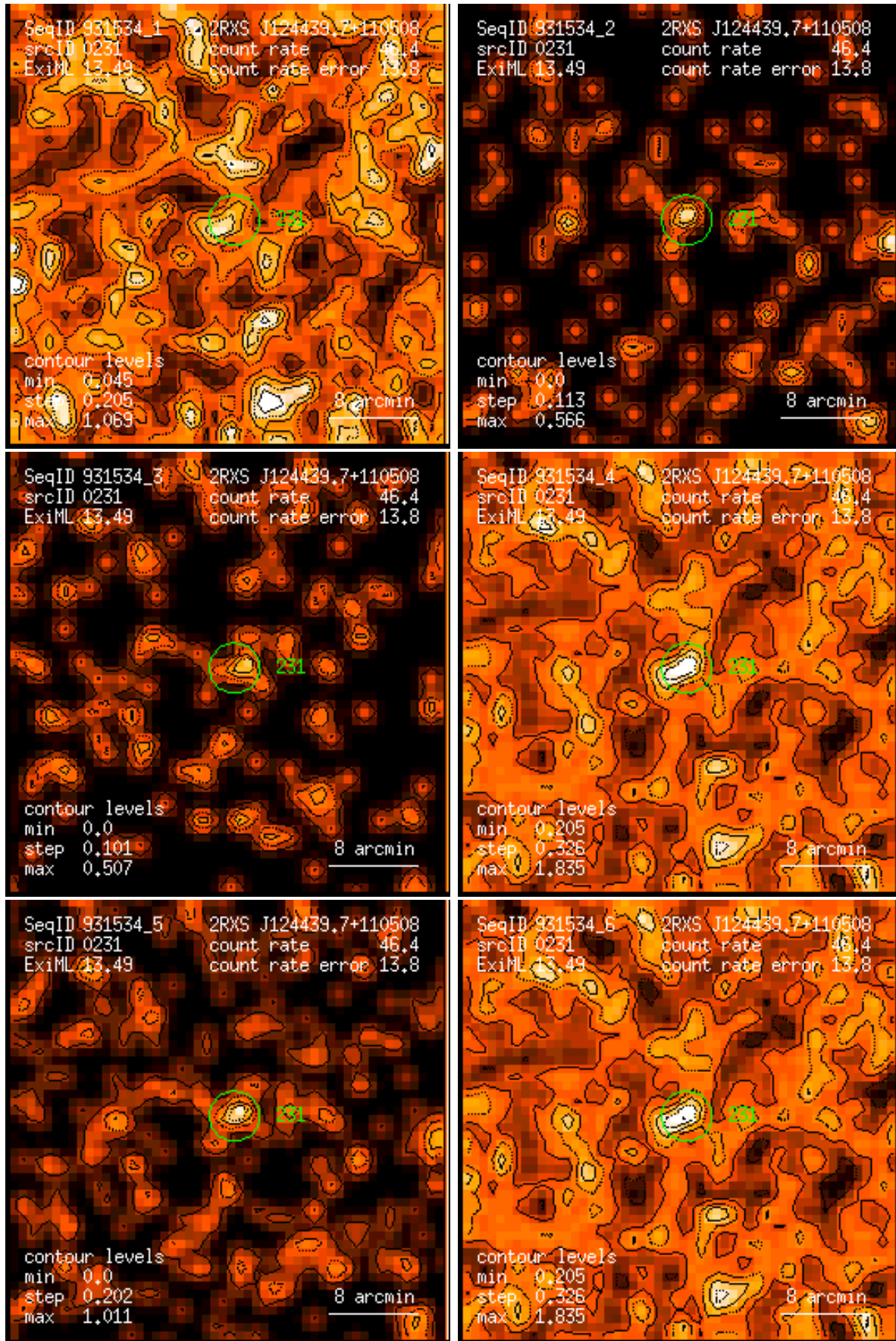
Figure 231: RASS 931534: detection 0231: band rate images, Gaussian filter: (1) PSPC channels 11 – 41, (2) 52 – 90, (3) 91 – 201, (4) 11 – 235, (5) 52 – 201, (6) 11 – 201. Broad band rates in counts/ks. Band rate contour levels in counts/ks/arcmin 2 .
