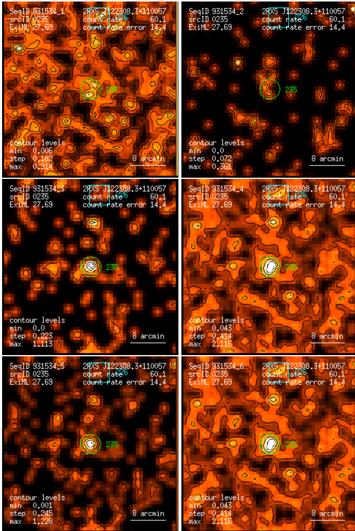
Figure 235: RASS 931534: detection 0235: band rate images, Gaussian filter: (1) PSPC channels 11 – 41, (2) 52 – 90, (3) 91 – 201, (4) 11 – 235, (5) 52 – 201, (6) 11 – 201. Broad band rates in counts/ks. Band rate contour levels in counts/ks/arcmin 2 .
