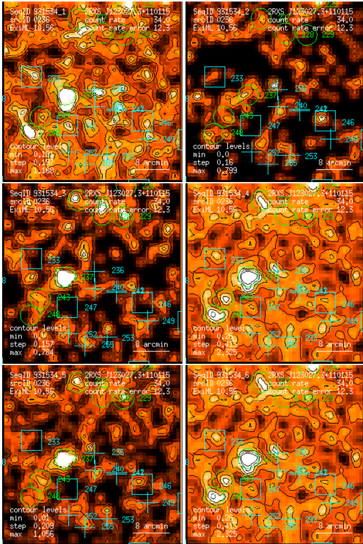
Figure 236: RASS 931534: detection 0236: band rate images, Gaussian filter: (1) PSPC channels 11 – 41, (2) 52 – 90, (3) 91 – 201, (4) 11 – 235, (5) 52 – 201, (6) 11 – 201. Broad band rates in counts/ks. Band rate contour levels in counts/ks/arcmin 2 .
