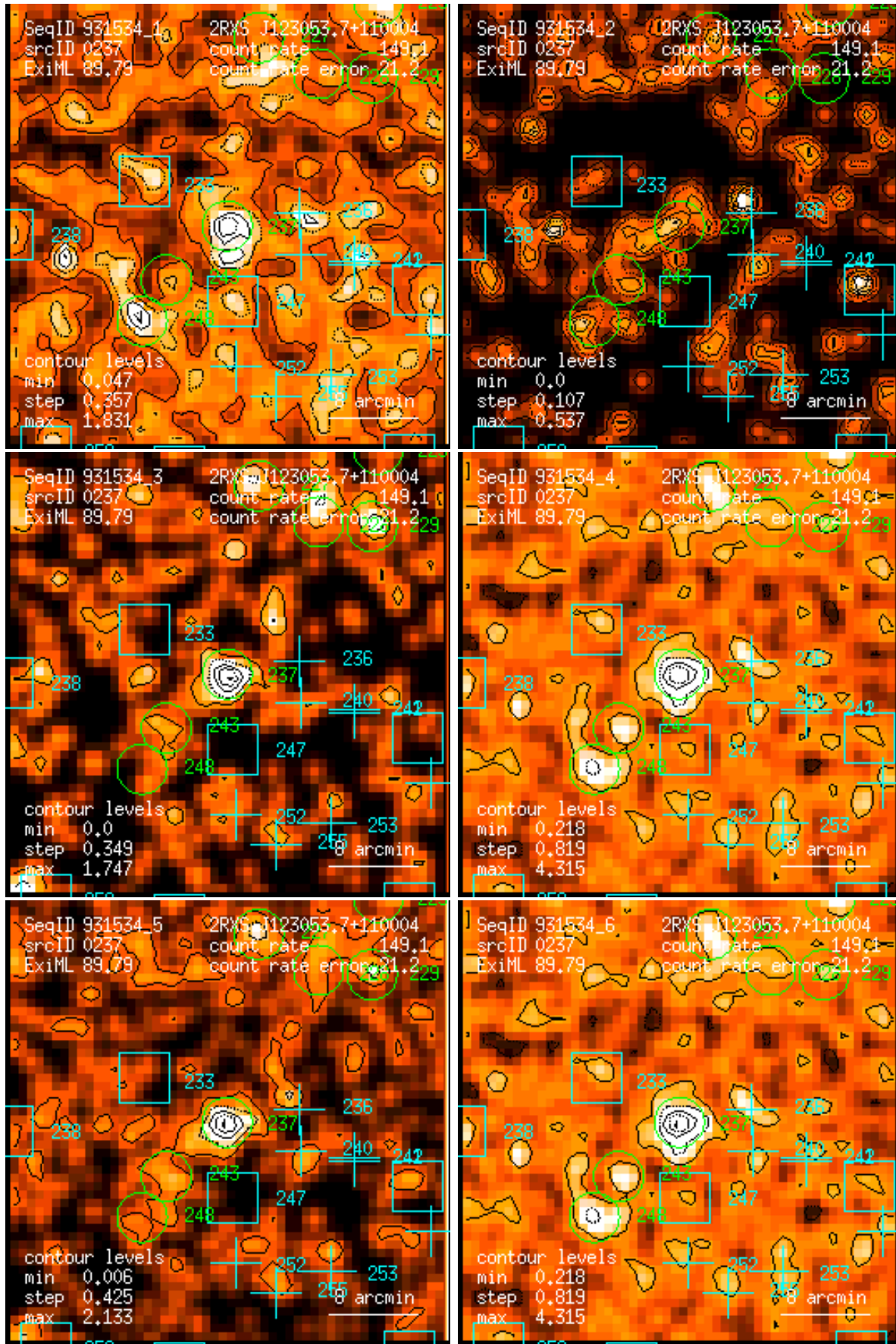
Figure 237: RASS 931534: detection 0237: band rate images, Gaussian filter: (1) PSPC channels 11 – 41, (2) 52 – 90, (3) 91 – 201, (4) 11 – 235, (5) 52 – 201, (6) 11 – 201. Broad band rates in counts/ks. Band rate contour levels in counts/ks/arcmin 2 .
