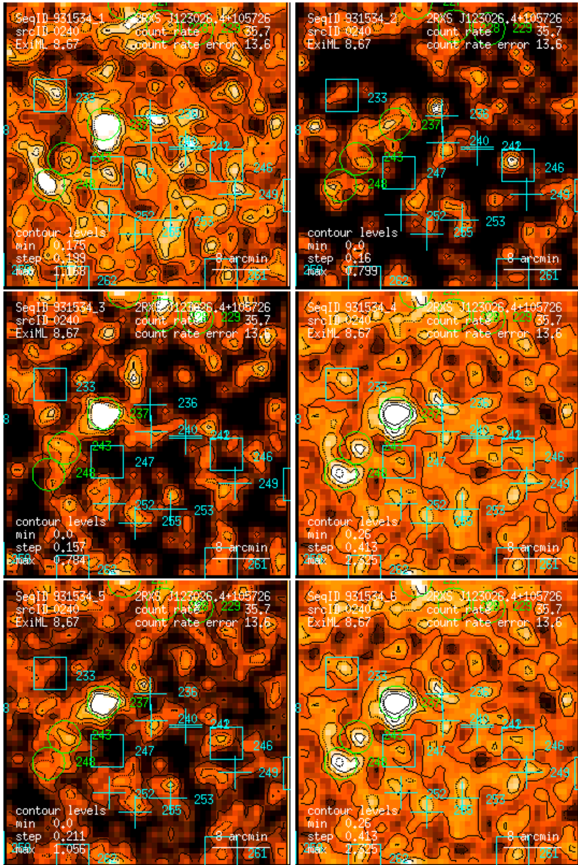
Figure 240: RASS 931534: detection 0240: band rate images, Gaussian filter: (1) PSPC channels 11 – 41, (2) 52 – 90, (3) 91 – 201, (4) 11 – 235, (5) 52 – 201, (6) 11 – 201. Broad band rates in counts/ks. Band rate contour levels in counts/ks/arcmin 2 .
