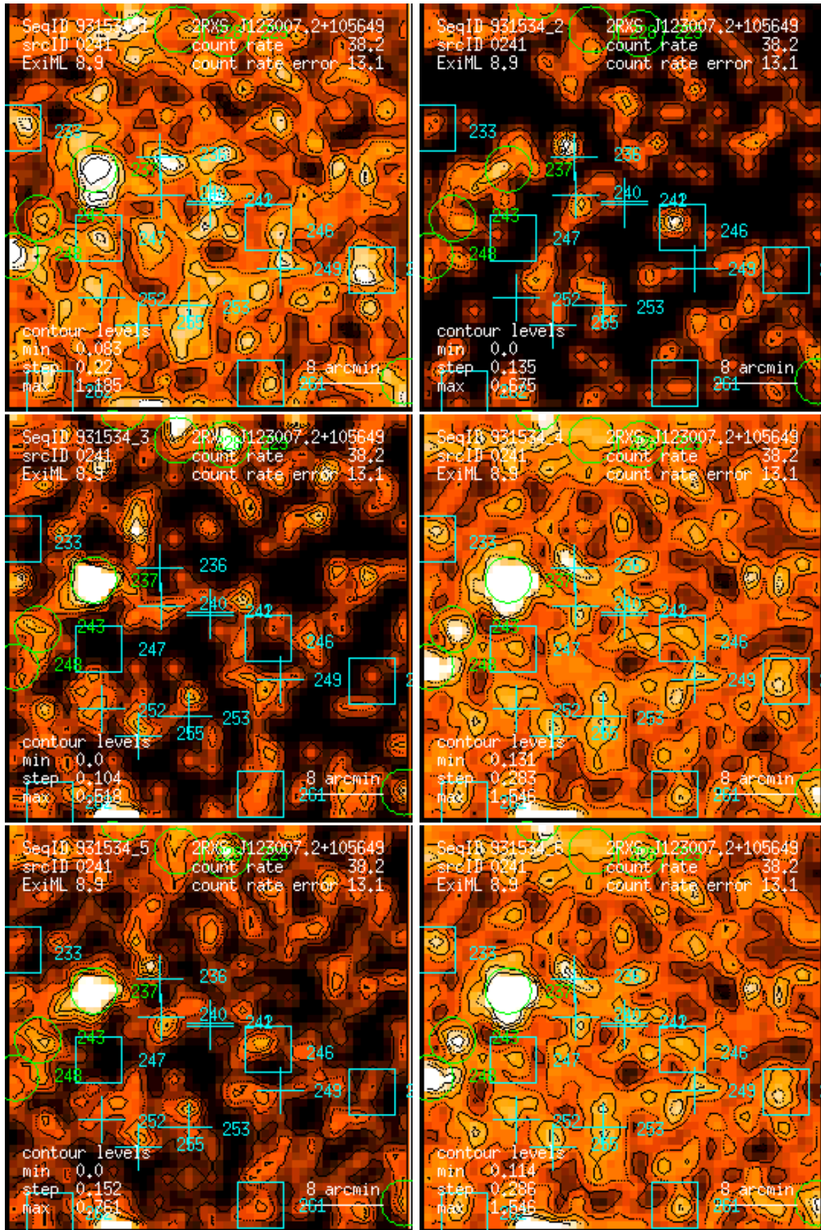
Figure 241: RASS 931534: detection 0241: band rate images, Gaussian filter: (1) PSPC channels 11 – 41, (2) 52 – 90, (3) 91 – 201, (4) 11 – 235, (5) 52 – 201, (6) 11 – 201. Broad band rates in counts/ks. Band rate contour levels in counts/ks/arcmin 2 .
