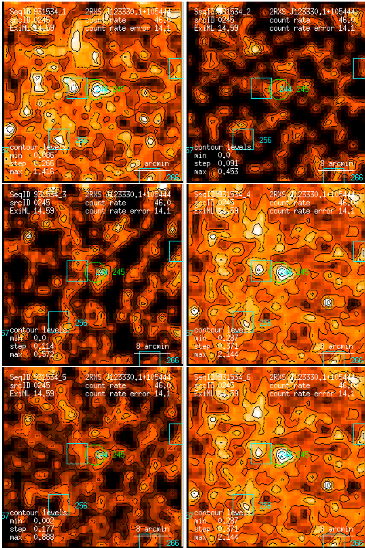
Figure 245: RASS 931534: detection 0245: band rate images, Gaussian filter: (1) PSPC channels 11 – 41, (2) 52 – 90, (3) 91 – 201, (4) 11 – 235, (5) 52 – 201, (6) 11 – 201. Broad band rates in counts/ks. Band rate contour levels in counts/ks/arcmin 2 .
