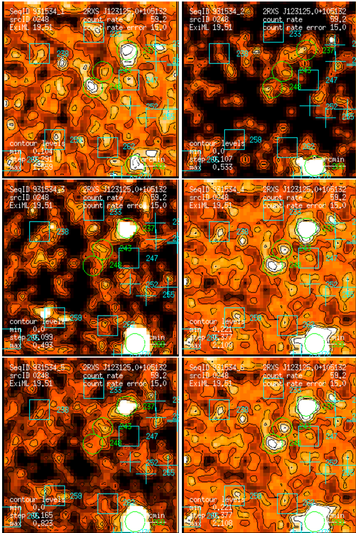
Figure 248: RASS 931534: detection 0248: band rate images, Gaussian filter: (1) PSPC channels 11 – 41, (2) 52 – 90, (3) 91 – 201, (4) 11 – 235, (5) 52 – 201, (6) 11 – 201. Broad band rates in counts/ks. Band rate contour levels in counts/ks/arcmin 2 .
