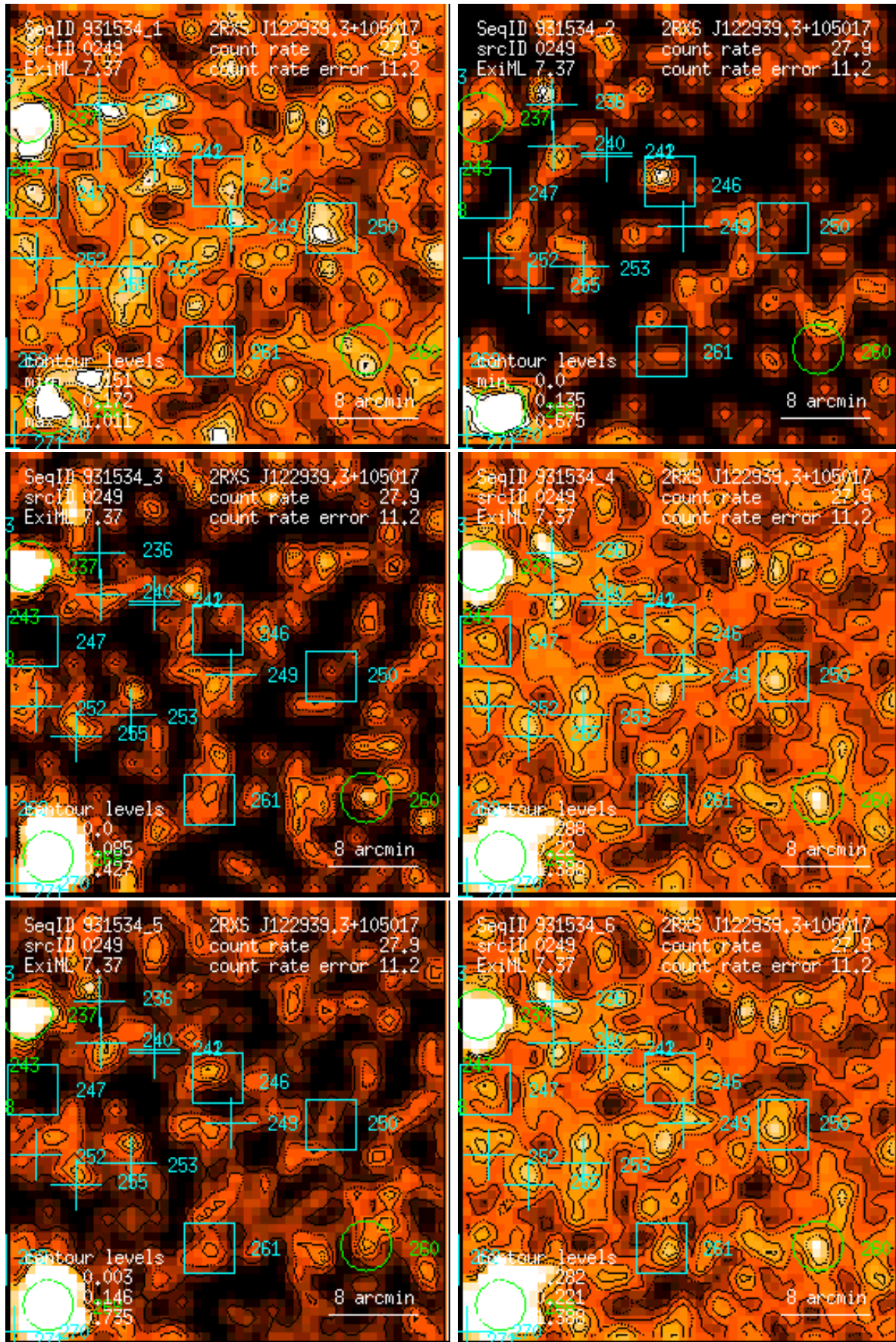
Figure 249: RASS 931534: detection 0249: band rate images, Gaussian filter: (1) PSPC channels 11 – 41, (2) 52 – 90, (3) 91 – 201, (4) 11 – 235, (5) 52 – 201, (6) 11 – 201. Broad band rates in counts/ks. Band rate contour levels in counts/ks/arcmin 2 .
