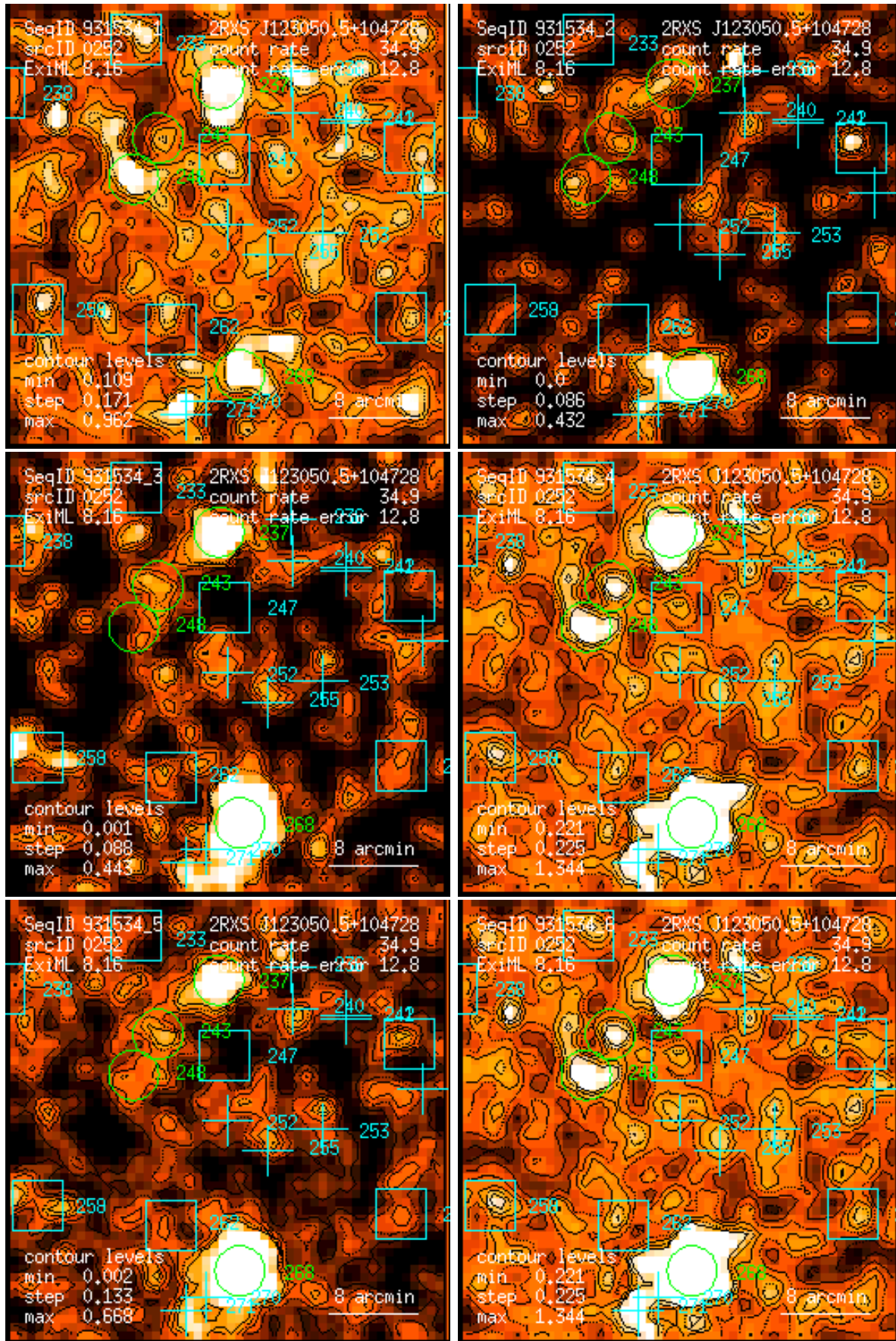
Figure 252: RASS 931534: detection 0252: band rate images, Gaussian filter: (1) PSPC channels 11 – 41, (2) 52 – 90, (3) 91 – 201, (4) 11 – 235, (5) 52 – 201, (6) 11 – 201. Broad band rates in counts/ks. Band rate contour levels in counts/ks/arcmin 2 .
