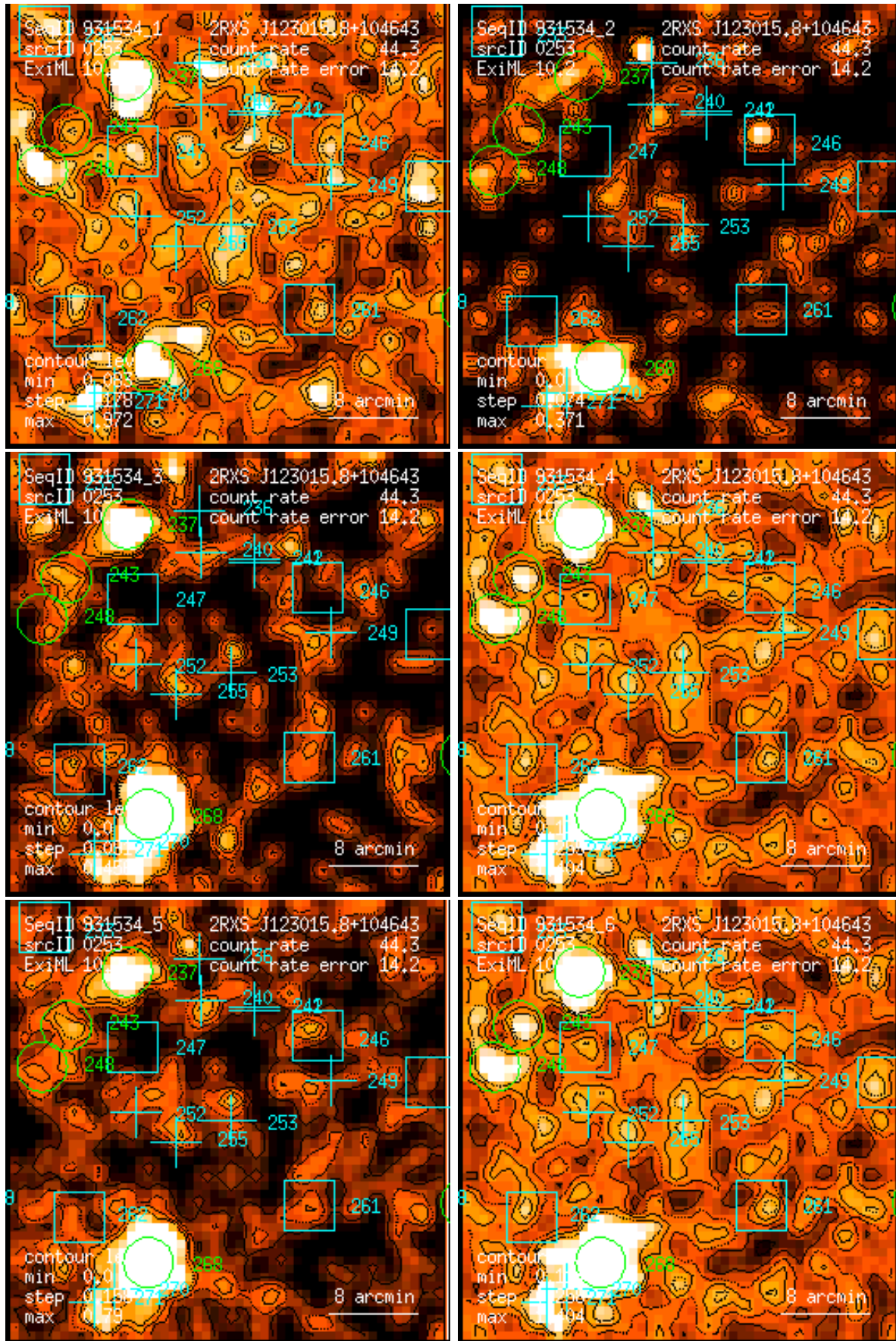
Figure 253: RASS 931534: detection 0253: band rate images, Gaussian filter: (1) PSPC channels 11 – 41, (2) 52 – 90, (3) 91 – 201, (4) 11 – 235, (5) 52 – 201, (6) 11 – 201. Broad band rates in counts/ks. Band rate contour levels in counts/ks/arcmin 2 .
