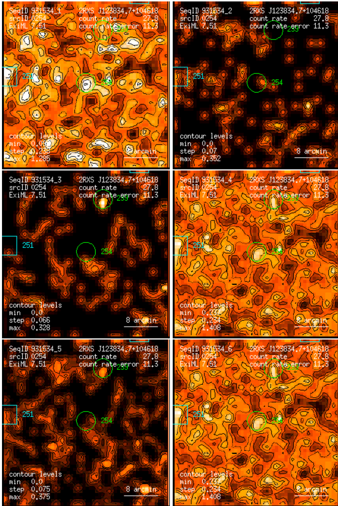
Figure 254: RASS 931534: detection 0254: band rate images, Gaussian filter: (1) PSPC channels 11 – 41, (2) 52 – 90, (3) 91 – 201, (4) 11 – 235, (5) 52 – 201, (6) 11 – 201. Broad band rates in counts/ks. Band rate contour levels in counts/ks/arcmin 2 .
