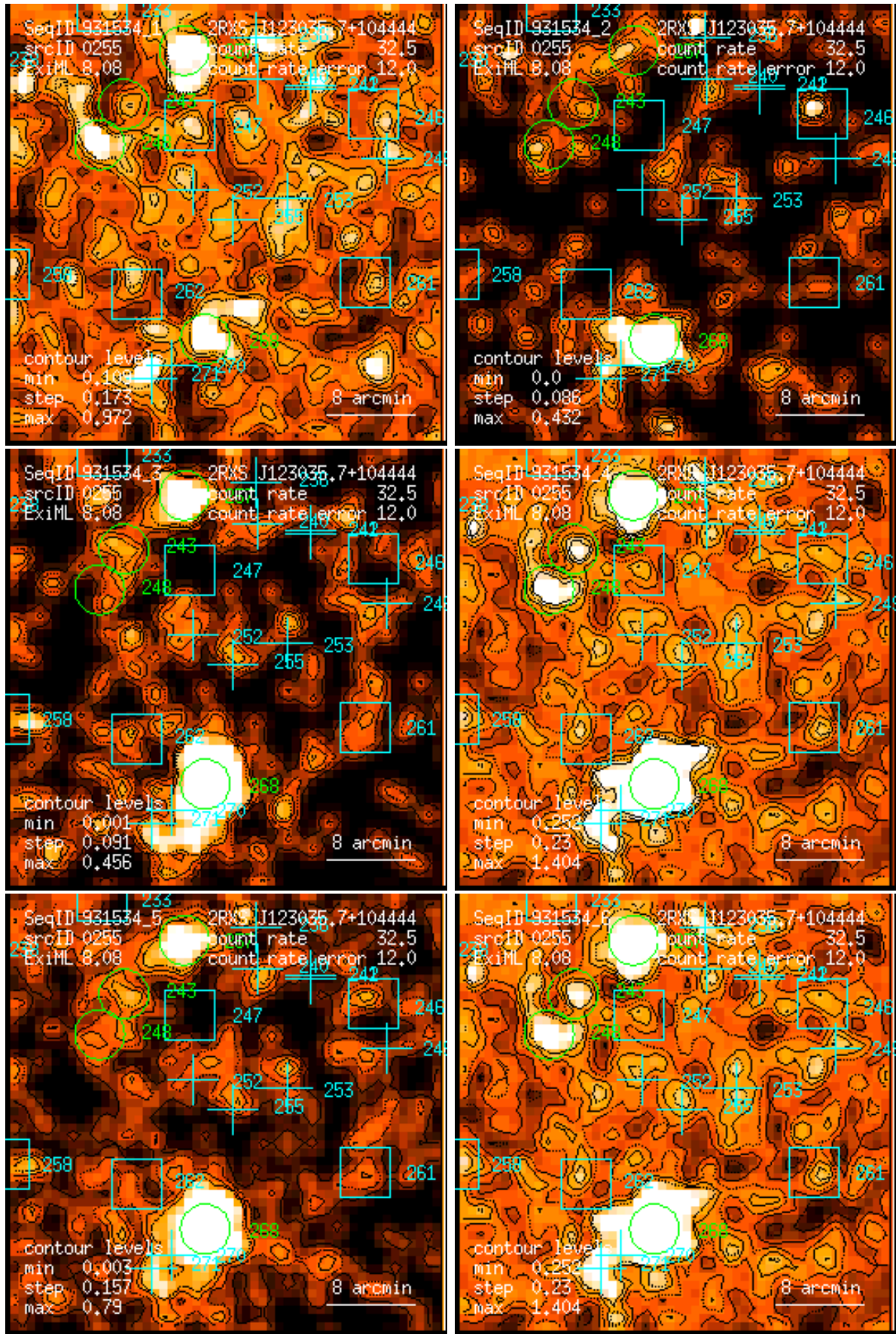
Figure 255: RASS 931534: detection 0255: band rate images, Gaussian filter: (1) PSPC channels 11 – 41, (2) 52 – 90, (3) 91 – 201, (4) 11 – 235, (5) 52 – 201, (6) 11 – 201. Broad band rates in counts/ks. Band rate contour levels in counts/ks/arcmin 2 .
