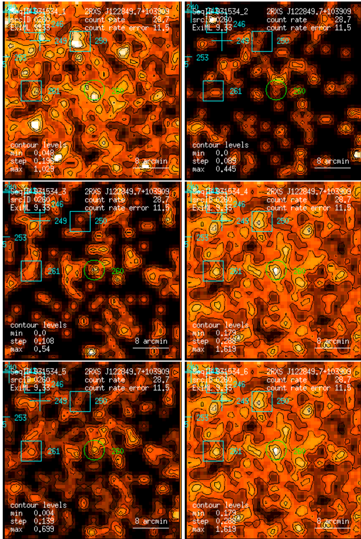
Figure 260: RASS 931534: detection 0260: band rate images, Gaussian filter: (1) PSPC channels 11 – 41, (2) 52 – 90, (3) 91 – 201, (4) 11 – 235, (5) 52 – 201, (6) 11 – 201. Broad band rates in counts/ks. Band rate contour levels in counts/ks/arcmin 2 .
