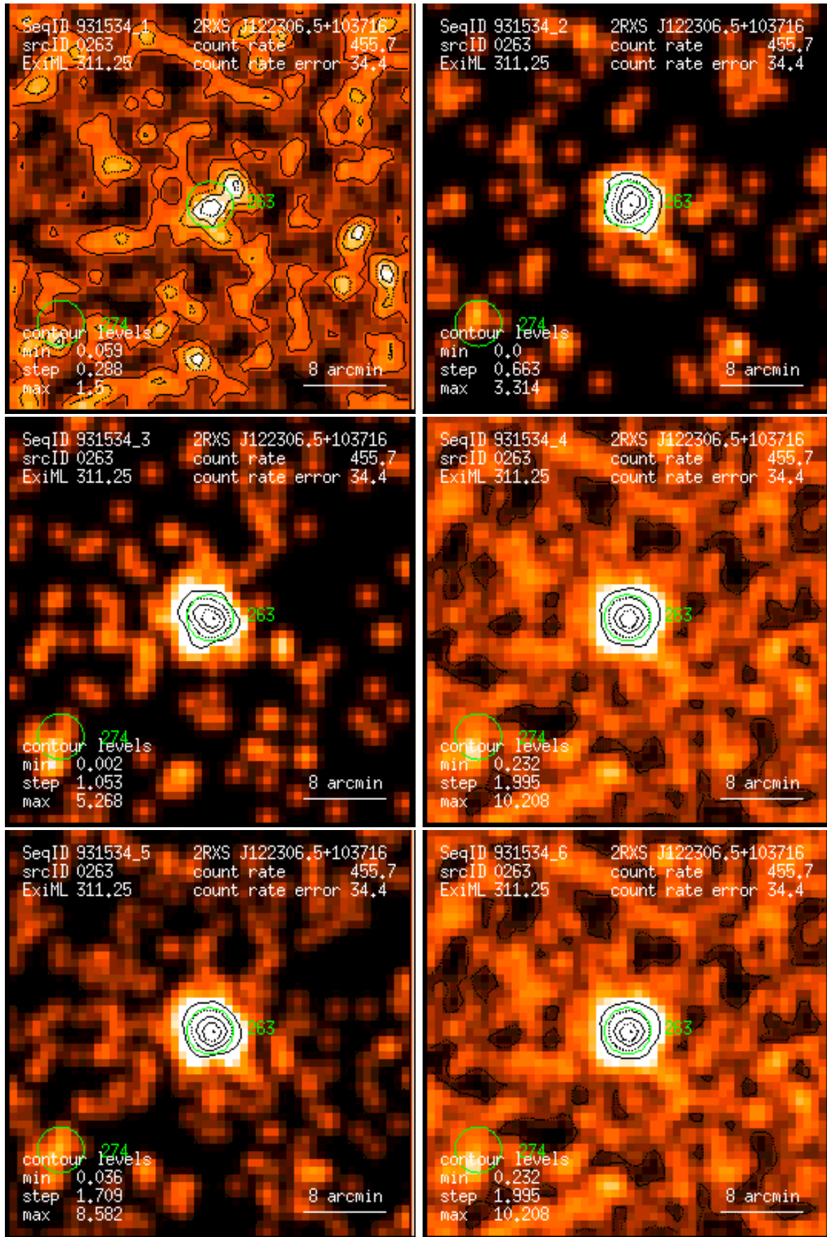
Figure 263: RASS 931534: detection 0263: band rate images, Gaussian filter: (1) PSPC channels 11 – 41, (2) 52 – 90, (3) 91 – 201, (4) 11 – 235, (5) 52 – 201, (6) 11 – 201. Broad band rates in counts/ks. Band rate contour levels in counts/ks/arcmin 2 .
