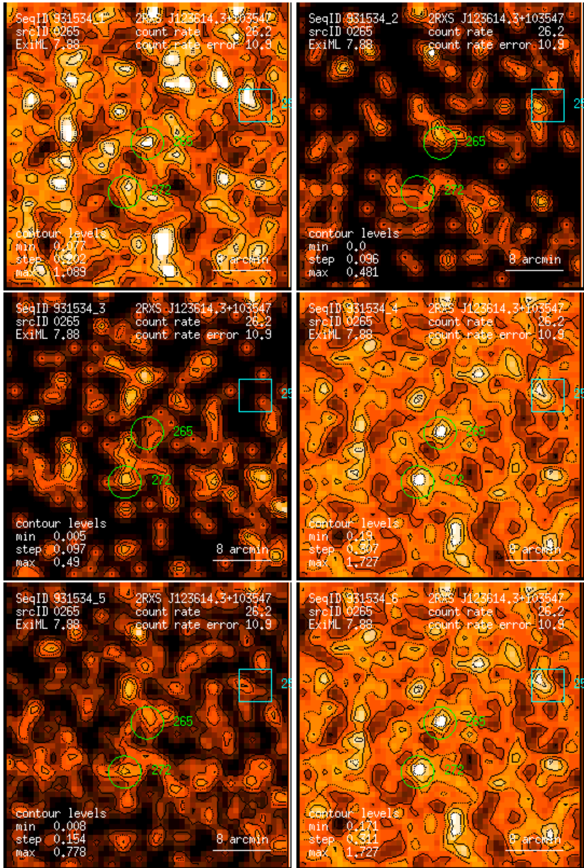
Figure 265: RASS 931534: detection 0265: band rate images, Gaussian filter: (1) PSPC channels 11 – 41, (2) 52 – 90, (3) 91 – 201, (4) 11 – 235, (5) 52 – 201, (6) 11 – 201. Broad band rates in counts/ks. Band rate contour levels in counts/ks/arcmin 2 .
