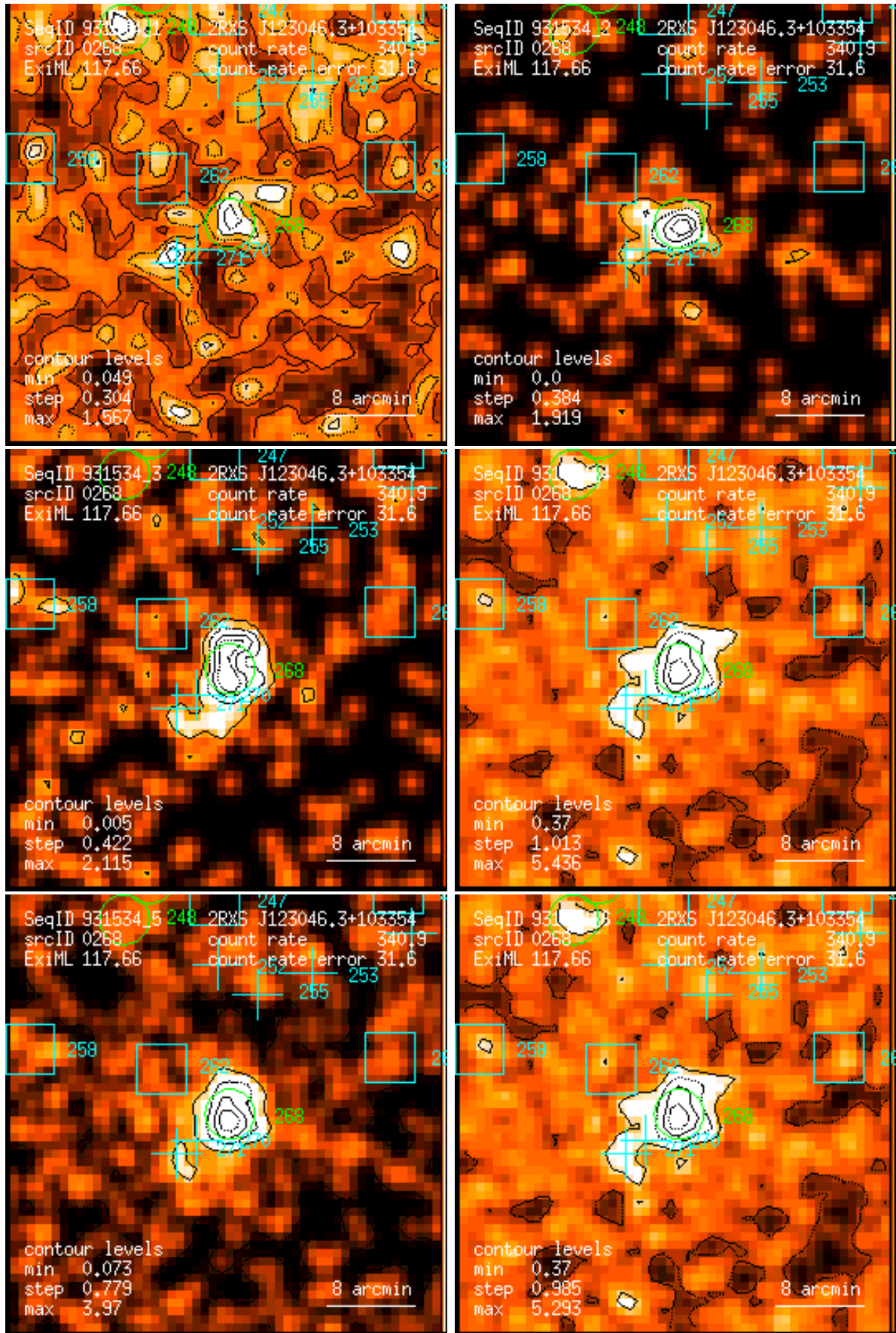
Figure 268: RASS 931534: detection 0268: band rate images, Gaussian filter: (1) PSPC channels 11 – 41, (2) 52 – 90, (3) 91 – 201, (4) 11 – 235, (5) 52 – 201, (6) 11 – 201. Broad band rates in counts/ks. Band rate contour levels in counts/ks/arcmin 2 .
