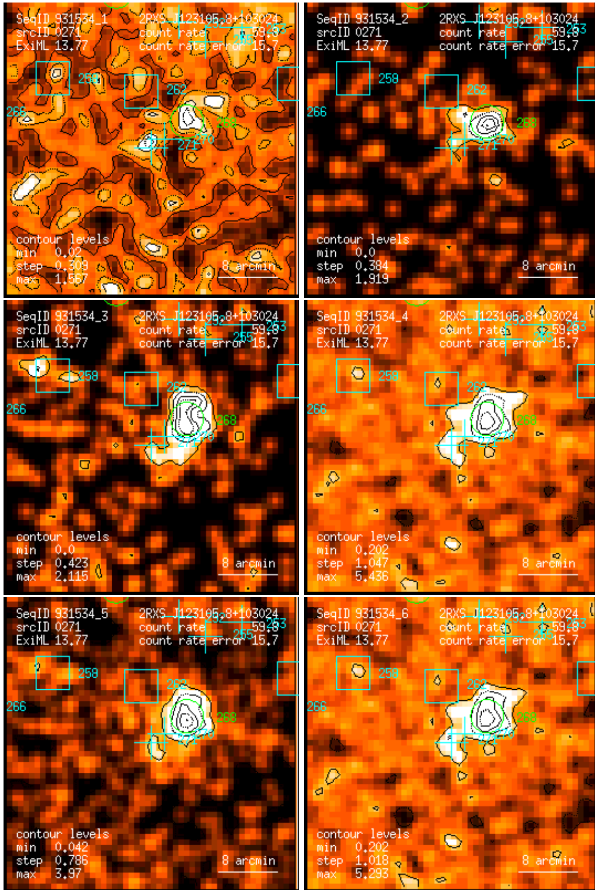
Figure 271: RASS 931534: detection 0271: band rate images, Gaussian filter: (1) PSPC channels 11 – 41, (2) 52 – 90, (3) 91 – 201, (4) 11 – 235, (5) 52 – 201, (6) 11 – 201. Broad band rates in counts/ks. Band rate contour levels in counts/ks/arcmin 2 .
